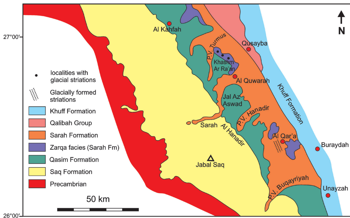
Fig. 2. Simplified geological map of the Al-Qassim Province, modified after Vaslet (1990)
