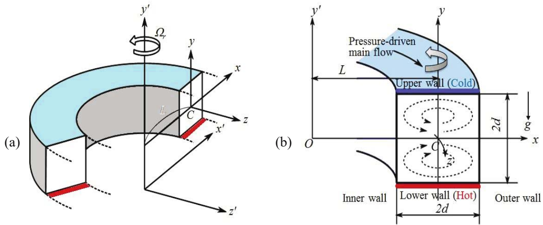
Fig.1. (a) Coordinate system of the curved duct, (b) Cross-section of the duct.
