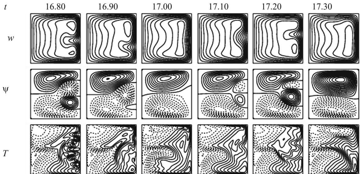
Fig.12. Streamlines of axial flow, secondary flow and temperature profiles for Tr = -30 .
