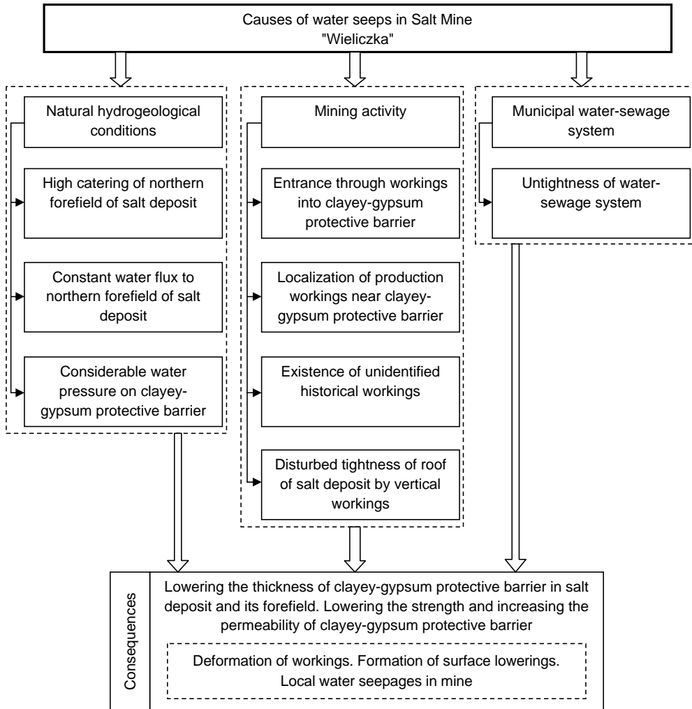
Fig. 2. Block diagram illustrating causes of water fluxes in the Salt Mine “Wieliczka”
