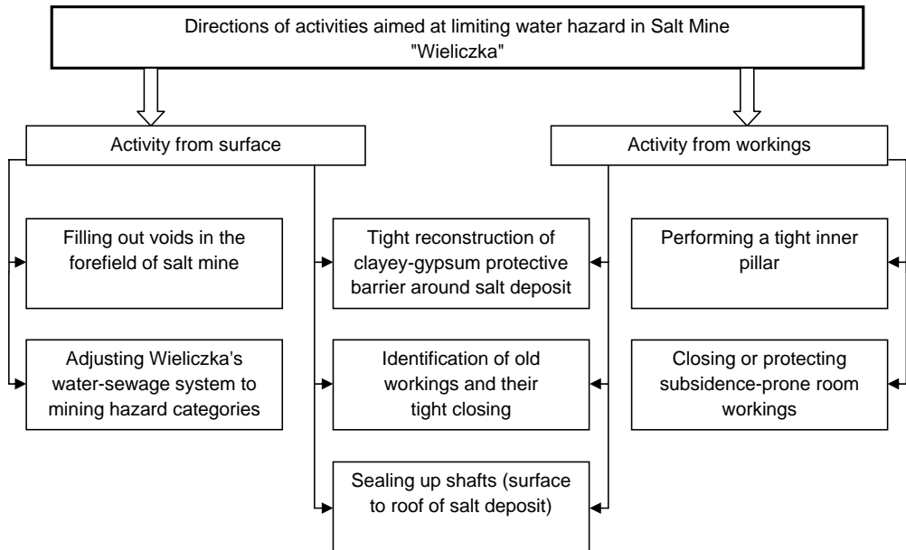
Fig. 3. Activities aimed at limiting water hazard in the Salt Mine "Wieliczka"
