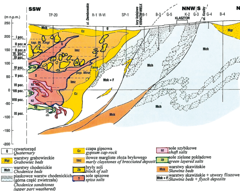
Fig. 1. Cross-section through the northern part of the mine in the transverse heading Mina area
