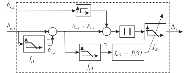
Fig. 5. Architecture of the i -th actuator health evaluator, AHE subsystem.
