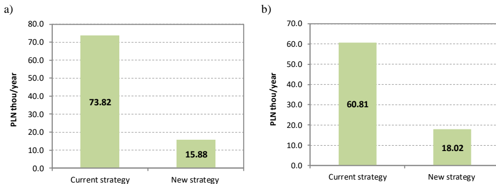
Fig. 3. Comparison of the costs of a P1 check annually at the current and the new strategies a) locomotive operated at Zakład Północny, b) locomotive operated at Zakład Śląski
