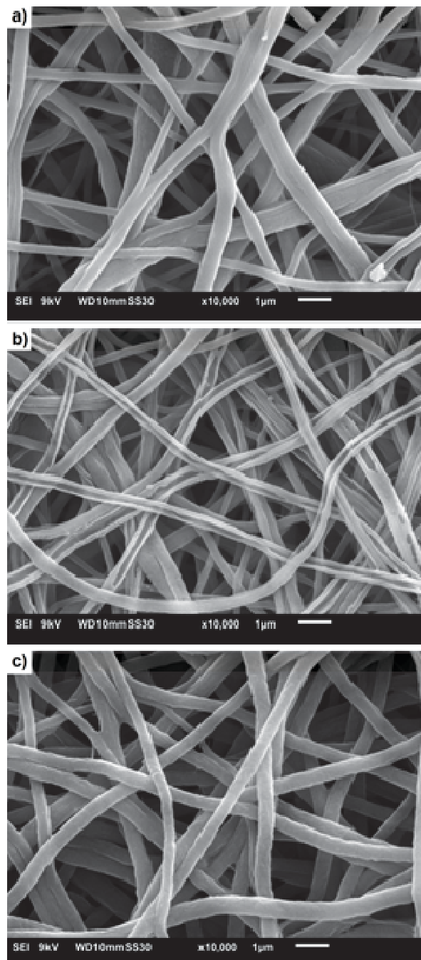
FIG. 1. Electrospun PCL/gelatin 7:3 material from acetic and formic acid mixture: a) not crosslinked, before biodegradation test; b) not crosslinked, after 30 days of biodegradation test; c) crosslinked, after 30 days of biodegradation test.
