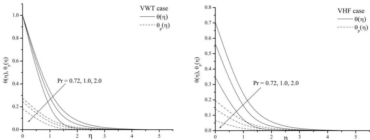
Fig.7a, b. The effect of the Prandtl number Pr on temperature distribution with A = 1.0, Ec = 1, R = 2, M = 0.1, N = 0.2, \beta = 1, Nr = 1, \lambda^* = 0.1 when \lambda = 0.5 .
