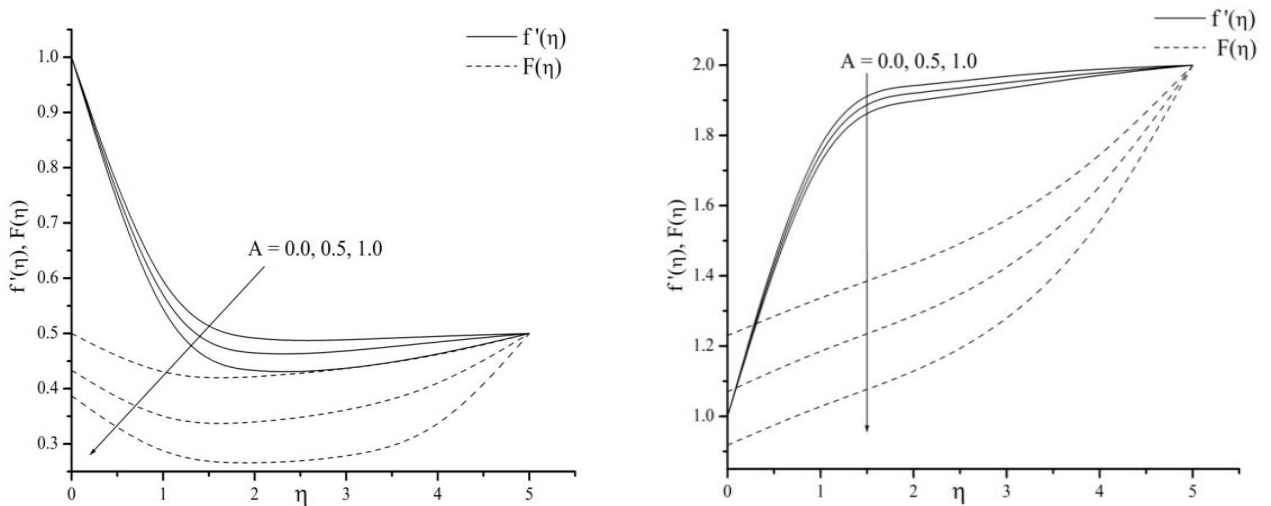
Fig.1a, b. The effect of the unsteady parameter A on the fluid and dust velocity with Pr=0.71, R=2, M=0.1, N=0.2, Nr=1 and \beta = 1.0, \lambda^* = 0.1 when \lambda = 0.5 and 2 .
