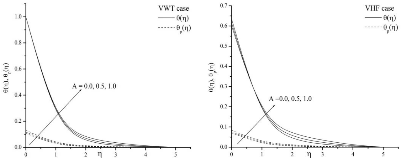
Fig.4a, b. The effect of the unsteady parameter A on temperature distribution with Pr = 0.71, Ec = 2, R = 0.5, M = 0.1, N = 0.2, \beta = 2, Nr = 1, \lambda^* = 0.1 when \lambda = 2 .
