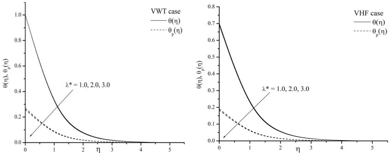
Fig.6a, b. The effect of the convective parameter \lambda^* on temperature distribution with A = 1.0, Pr = 0.71, Ec = 1, R = 2, M = 0.1, N = 0.2, Nr = 1, \beta = 1 , when \lambda = 0.5 .
