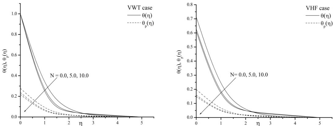
Fig.9a, b. The effect of the number density N on temperature distribution with A = 1.0, Pr = 0.71, R = 2, M = 0.1, Ec = 1, \beta = 1, Nr = 1, \lambda^* = 0.1 when \lambda = 0.5 .
