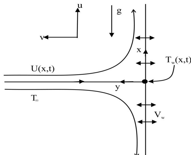
Figure: Schematic diagram of the flow geometry.
