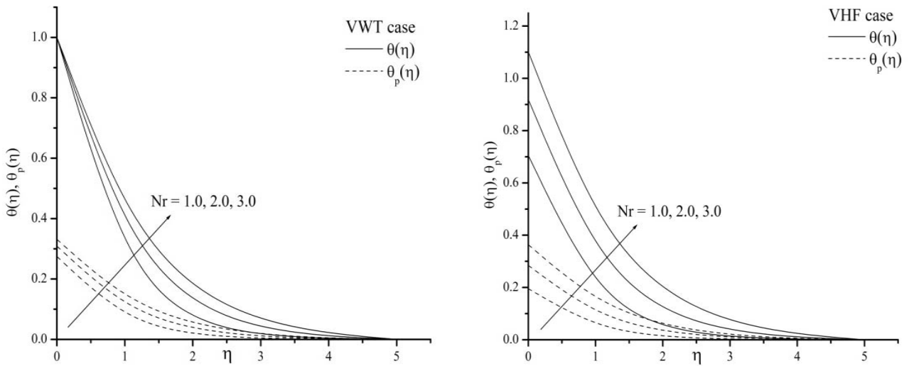
Fig.10a, b. The effect of the thermal radiation parameter Nr on temperature distribution with A = 1.0, Pr = 0.71, R = 2, M = 0.1, Ec = 1, \beta = 1, \lambda^* = 0.1 when \lambda = 0.5 .
