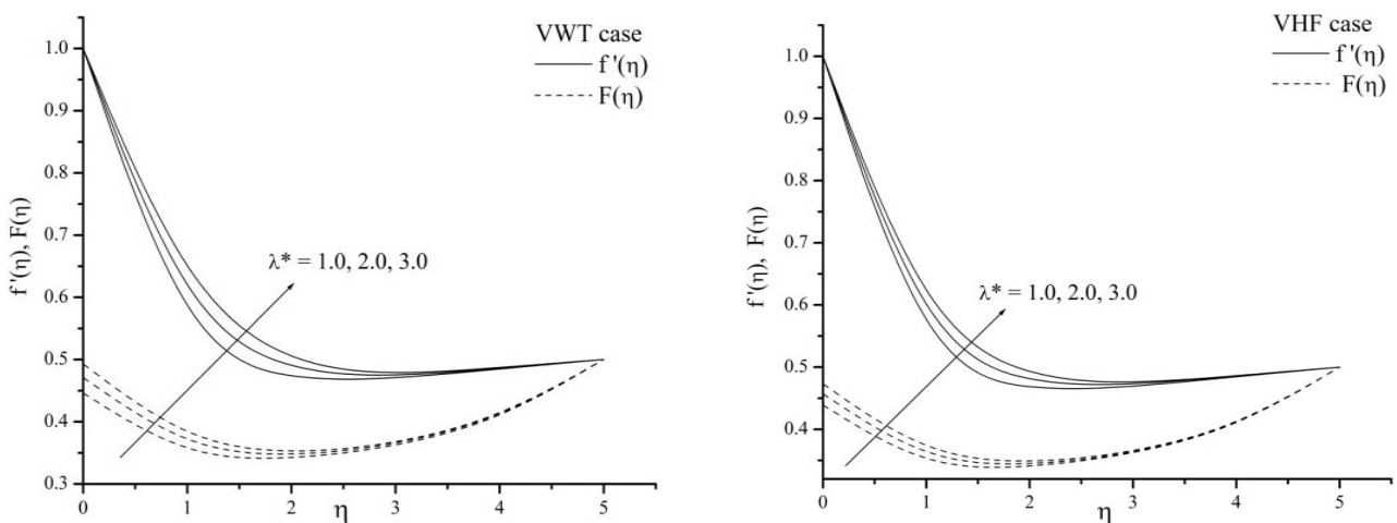
Fig.5a, b. The effect of the convective parameter \lambda^* on fluid and dust velocity A = 1.0, Pr = 0.71, Ec = 1, R = 2, M = 0.1, N = 0.2, \beta = 1, Nr = 1 when \lambda = 0.5 .
