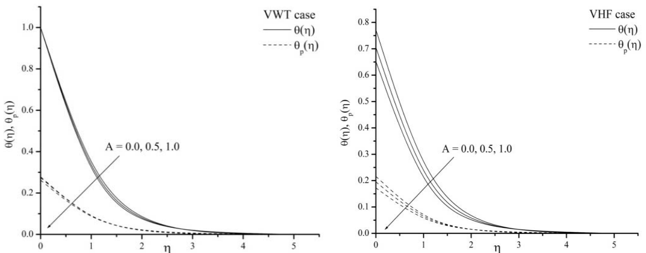
Fig.3a, b. The effect of the unsteady parameter A on temperature distribution with Pr = 0.71, Ec = 2, R = 2, M = 0.1, N = 0.2, \beta = 1, \lambda^* = 0.1, Nr = 1 when \lambda = 0.5 .
