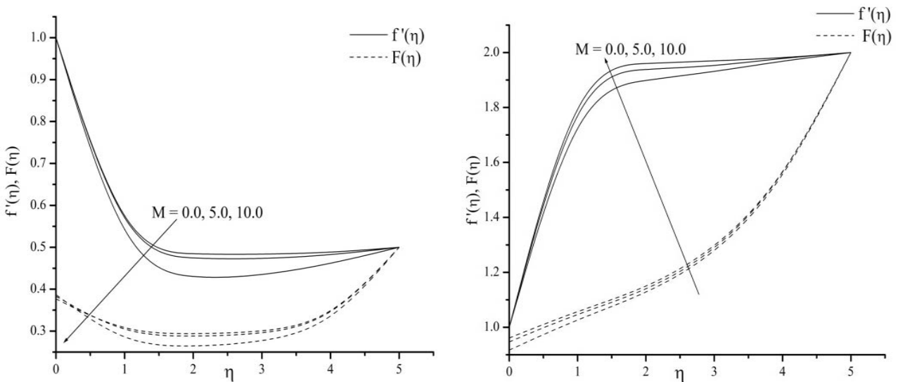
Fig.2a, b. The effect of the Hartman number M on the fluid and dust velocity with Pr=0.71, R=2, Ec=1, N=0.2, \beta = 1.0, Nr=1 and \lambda^* = 0.1 , when \lambda = 0.5 and 2 .
