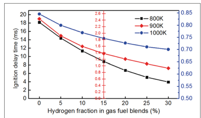
Fig.4. Ignition delay times versus varying hydrogen ratios at different temperatures in numerical simulations
