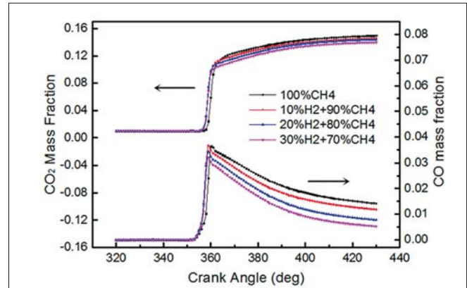
Fig.13. Effect of varying hydrogen ratios on CO and CO 2 emissions versus crank angle behaviour in numerical simulations
