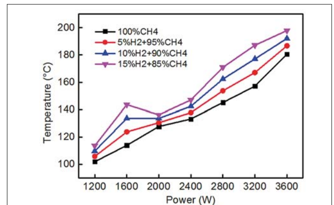
Fig. 9. Effect of varying hydrogen ratios on exhaust gas temperatures versus power behaviour in experiments
