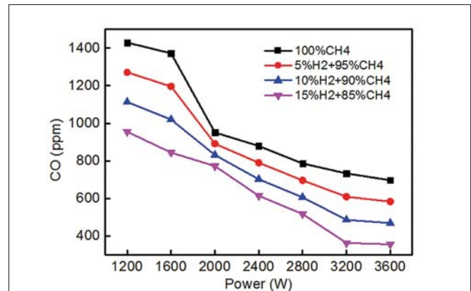
Fig.15. Effect of varying hydrogen ratios on CO concentration versus power behaviour in experiments
