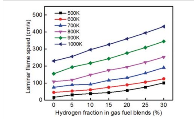
Fig.5. Laminar flame speeds versus varying hydrogen ratios at different temperatures in numerical simulations
