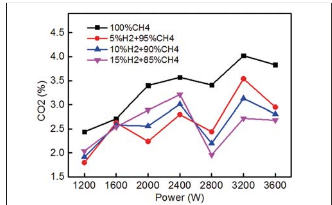
Fig.14. Effect of varying hydrogen ratios on CO 2 concentration versus power behaviour in experiments
