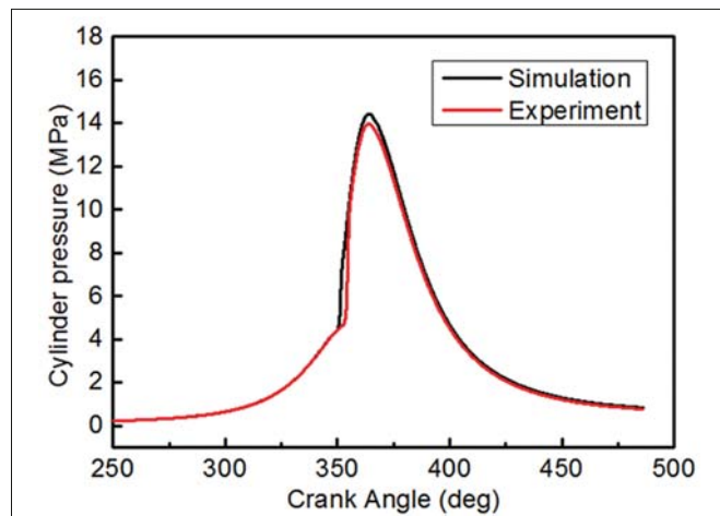
Fig.2. Comparison of experimental and calculated cylinder pressure values
