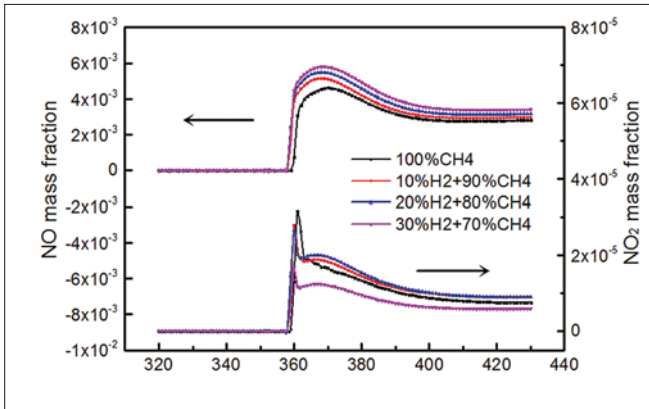
Fig.10. Effect of varying hydrogen ratios on NO and NO 2 emissions versus crank angle behaviour in numerical simulations
