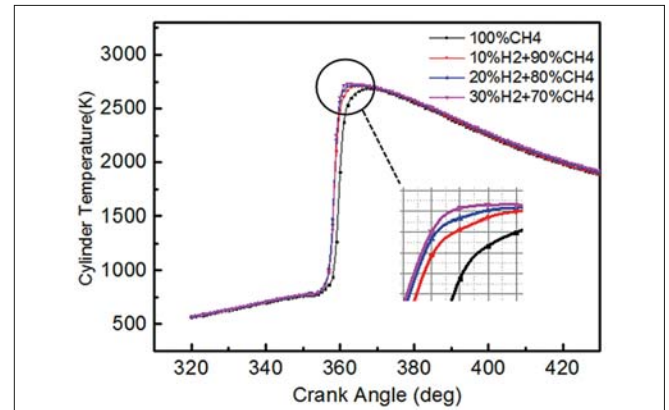
Fig. 8. Effect of varying hydrogen ratios on in-cylinder temperature versus crank angle behaviour in numerical simulations
