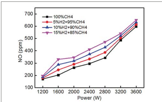
Fig. 12. Effect of varying hydrogen ratios on NO concentration versus power behaviour in experiments
