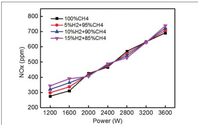
Fig.11. Effect of varying hydrogen ratios on NO x concentration versus power behaviour in experiments
