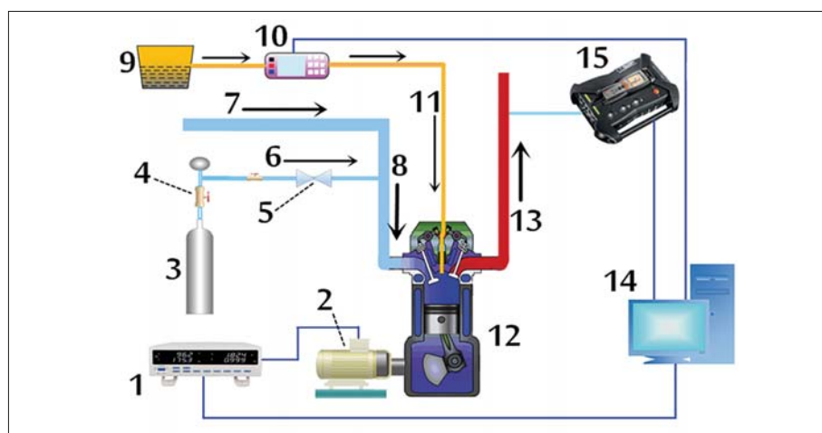
Fig.3. Diagram of the experimental system // 1. Dynamometer control cabinet, 2. Permanent magnet synchronous dynamometer, 3. Cylinder filled with gas fuel ( CH_4 + H_2 ), 4. Flow regulating valve, 5. Check valve, 6. Intake manifold ( CH_4 + H_2 ), 7. Fresh air duct tube, 8. Intake main, 9. Fuel tank, (diesel), 10. Fuel consumption monitor, 11. Fuel rail, 12. Single-cylinder engine, 13. Exhaust emission, 14. Computers for control and data collection, 15. Testo 350 combustion gas analyser
