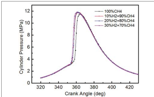
Fig. 7. Effect of varying hydrogen ratios on in-cylinder pressure versus crank angle behaviour in numerical simulations
