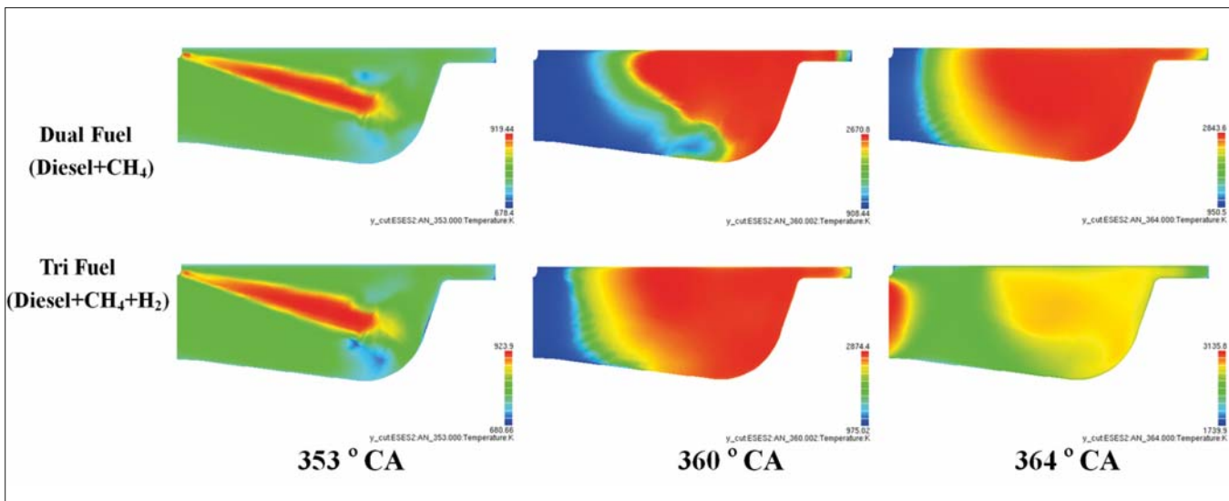
Fig. 6. Temperature distribution of the engine's cylinder at top dead centre positions under different hydrogen ratios
