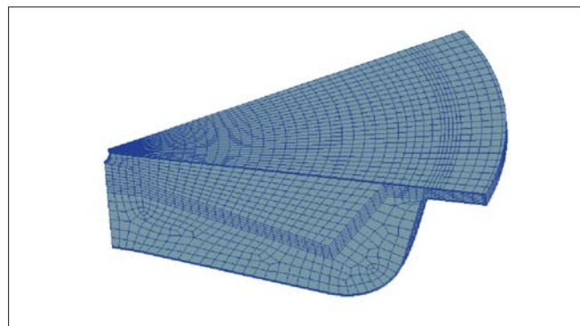
Fig. 1. Sector meshes used in engine simulation
