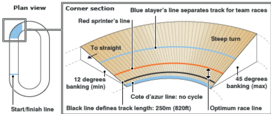
Fig. 2. Scheme of the construction of the cycling track; source: www.bbc.com , access: 20.08.2015
