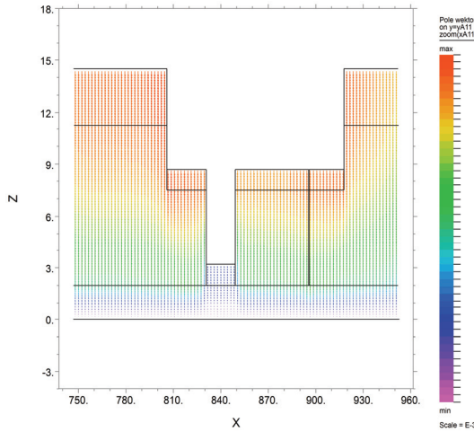
Fig. 12. Vectorial field of vertical displacements in the cross-section A1-A1'. (Displacements are expressed in meters; scale multiplier = 1e-3)
