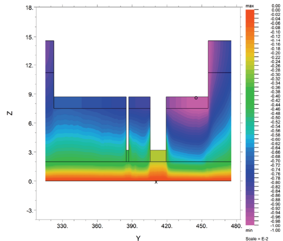
Fig. 15. The settlements of the system soil-slab in the cross-section B1-B1'. (Settlements are expressed in meters; scale multiplier = 1e-2)
