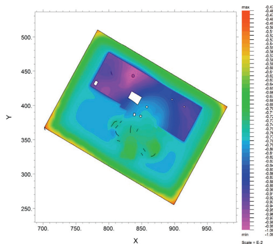
Fig. 9. Isolines of settlement of the top surface of the foundation slab. (Settlement is expressed in meters; scale multiplier = 1e-2)
