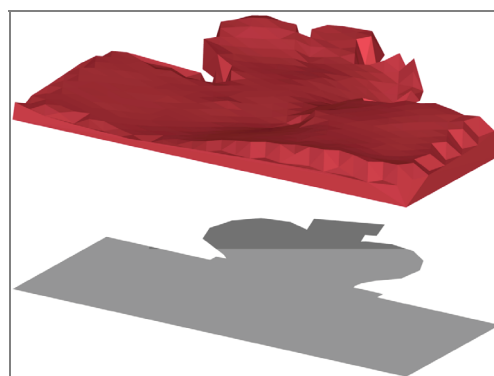
Fig. 10. A spatial image of settlements of the foundation slab
