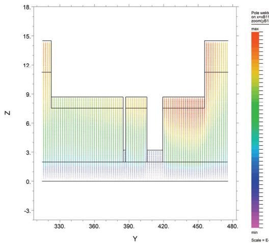
Fig. 13. Vectorial field of vertical displacements in the cross-section B1-B1'. (Displacements are expressed in meters; scale multiplier = 1e-3)
