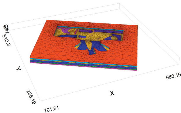
Fig. 4b. Spatial image of the numerical model used to predict settlement of soils and foundation slab deformations
