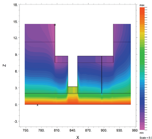
Fig. 14. The settlements of the system soil-slab in the cross-section A1-A1'. (Settlements are expressed in meters; scale multiplier = 1e-3)
