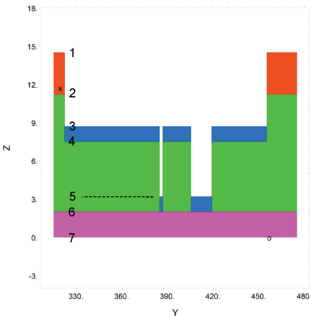
Fig. 7. Distribution of computing layers in the cross-section south-north B1-B1'. (More detailed description is in the text)
