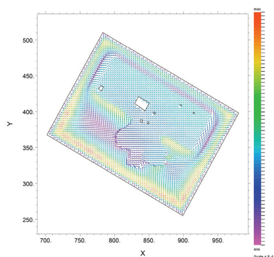
Fig. 11. The vectorial field of horizontal displacements at the top of the foundation slab. (Displacements are expressed in meters; scale multiplier = 1e-4)
