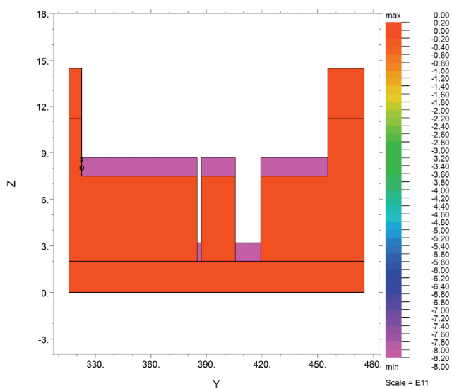
Fig. 8. Plastic potential in the cross-section B1-B1' according to the Drucker–Prager criterion
