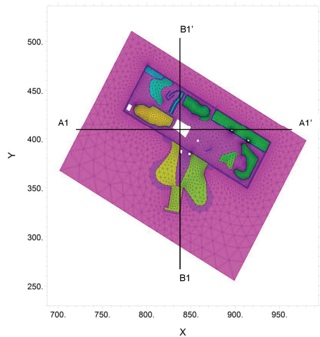
Fig. 5. Mesh of finite elements at the level of the slab. Scheme of slab load; different colours represent different types and values of load. White areas represent the lower level of the slab
