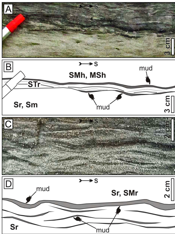
Fig. 5. Wavy bedding. A, B – wavy bedding at the boundary between the ripple cross-laminated sands and horizontally laminated muddy-sandy sediments; C, D – wavy bedding situated predominantly within rippled sandy deposits with a muddy admixture. Note the relatively continuous muddy layers that drape the sandy ripple structures; flow direction is almost perpendicular to the photograph; for explanation of lithofacies code see text and Table 1
