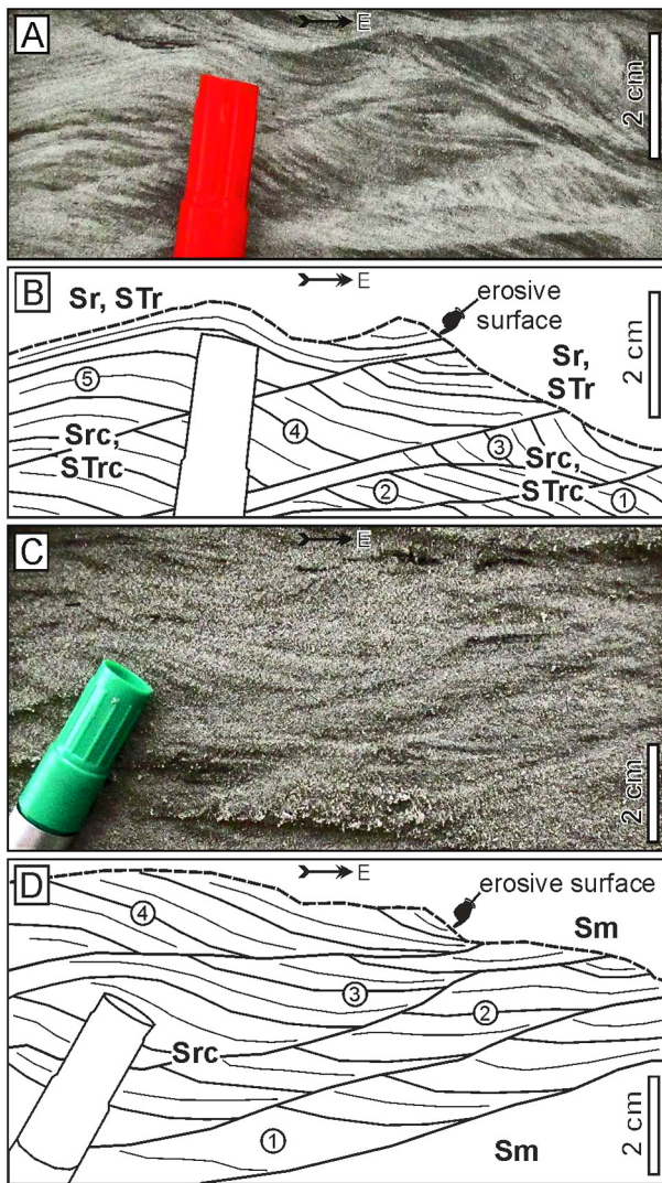
Fig. 3. Climbing-ripple cross-lamination. A, B – Sand and sandy-silt with climbing ripples; C, D – Sand with climbing ripples. Note the low angle of climb ( < 10^\circ ) in both examples; flow direction is from left to right, numerals in circles indicate successive generations of climbing ripples; for explanation of lithofacies code see text and Table 1
