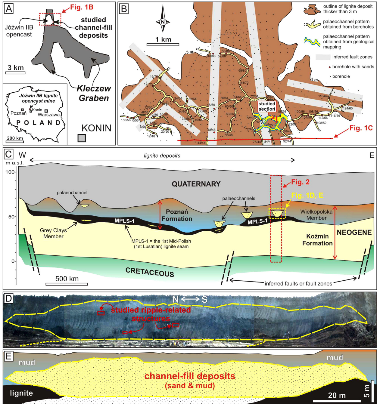
Fig. 1. Localities and geology of the study area. A – Map of the Konin area in central Poland showing the location of the Józwin IIB lignite opencast mine in the Kleczew Graben area; B – Palaeochannel pattern inferred from borehole data and geological mapping in the area of the Państw IV lignite deposits (modified from Widera et al., 2017); C – Simplified geological cross-section through the northern segment of the Kleczew Graben (the southernmost part of the Państw IV lignite deposits) with the approximate stratigraphical position of the palaeochannel studied (modified from Widera, 2014, Widera et al., 2017); D, E – Broad view and corresponding line-drawings of the palaeochannel. Note the location of the ripple-related structures within the palaeochannel examined
