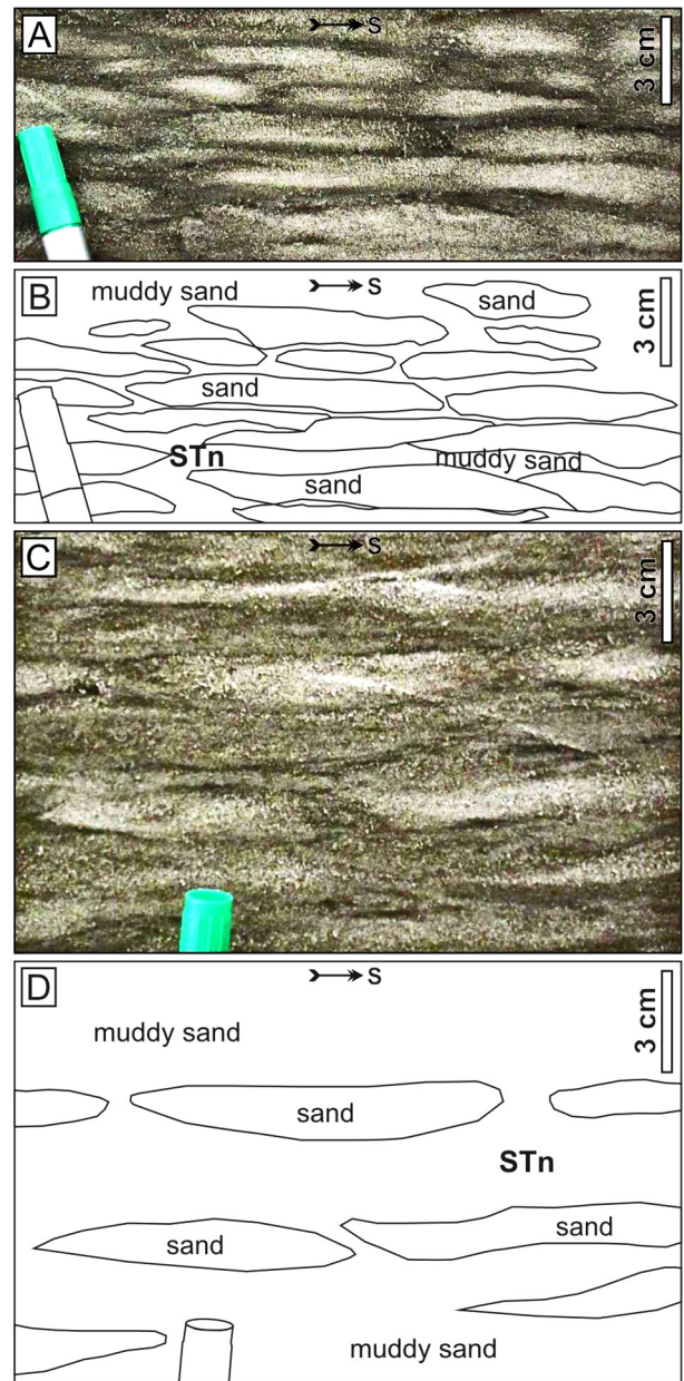
Fig. 6. Lenticular (nodular) bedding. A, B – lenticular bedding with a predominance of ‘lens-like’ sands; C, D – lenticular bedding with a predominance of muddy-sandy matrix. Note that ‘lens-like’ sands are surrounded by muddy sand; flow direction is almost perpendicular to the photograph; for explanation of lithofacies code see text and Table 1
