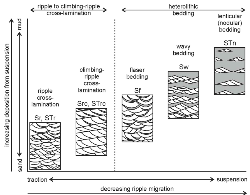
Fig. 8. Simplified diagram showing the relationship between traction and suspension processes, as well as between sand and mud content during formation of ripple-derived sedimentary structures. For explanation of lithofacies code see text and Table 1.
