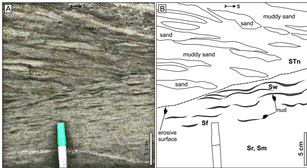
Fig. 7. Co-occurrence of various types of heterolithic bedding. Note the upward transition from flaser (Sf), through wavy (Sw) to lenticular (STn) bedding within the sedimentary succession; flow direction is almost perpendicular to the photograph; for explanation of lithofacies code see text and Table 1
