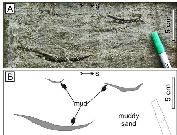
Fig. 4. Flaser bedding. Note the discontinuous muddy layers, consisting of muddy infill of ripple troughs, surrounded by poorly laminated muddy sand. Note that discontinuous 'lens-like' muddy layers surrounded by muddy sand; flow direction is almost perpendicular to the photograph; for explanation of lithofacies code see text and Table 1
