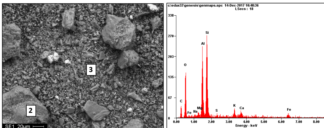
Fig. 3. SEM and EDX analyses of the ash from the coke breeze. 1 – surface analysis
