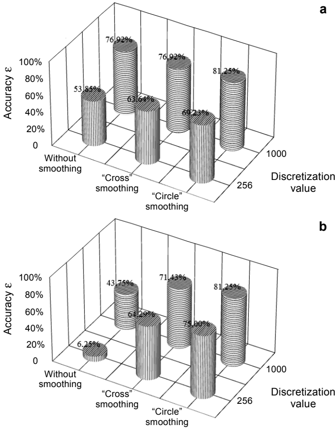
Fig. 6. Exactness of singularity reconstruction for images with the size of 200×200 (a) and 600×600 (b) at different intensity discretization and different smoothing procedures.
