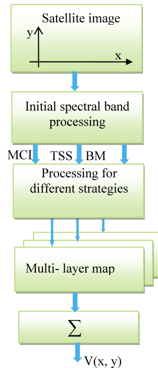
Fig. 2. Remote sensing flow chart.
