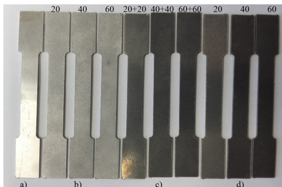
Fig. 7. The samples a) before machining, b) after deburring on 20, 40, 60 min, c) after deburring on 20 + polishing on 20 min, 40 min, 60 min, d) after polishing on 20, 40 min, 60 min
