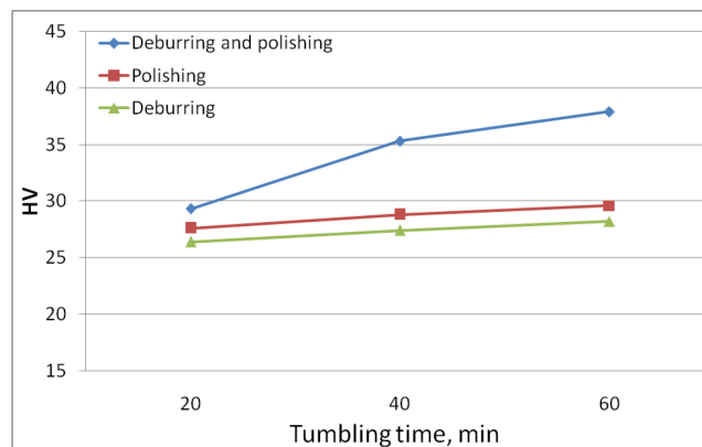
Fig. 6. Graph of hardness dependence ( HV ) on the duration of vibratory machining
