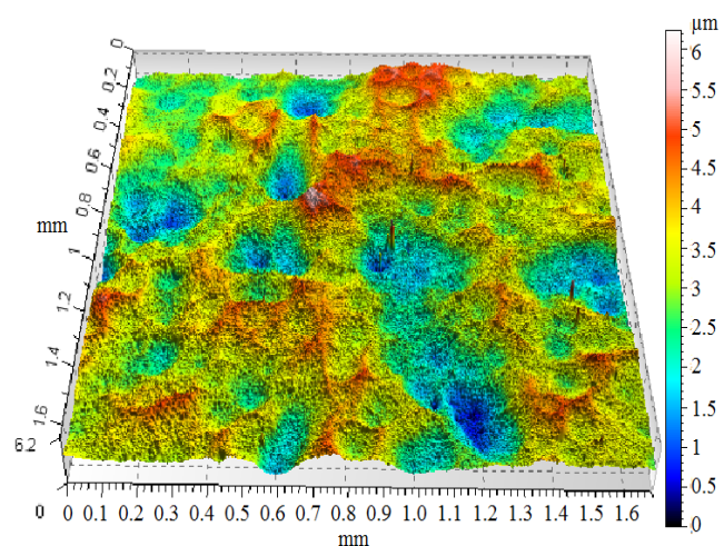
Fig. 11. 3D optical surfaces of the sample after vibro-abrasive deburring on 60 min. and polishing on 60 min; S_a = 0.6365 \mu\text{m}
