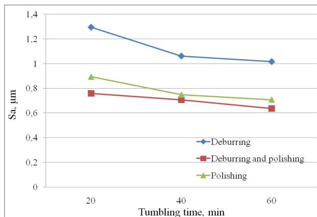
Fig. 4. Graph of the average surface roughness S_a on the duration of vibratory machining
