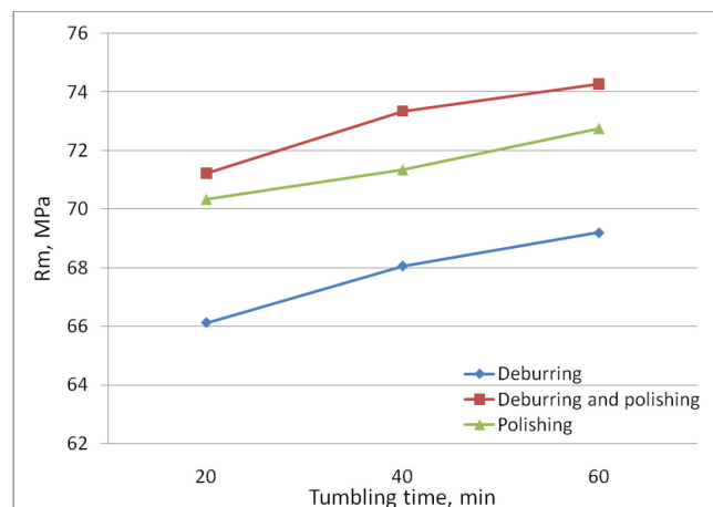
Fig. 5. Graph of tensile strength ( R_m ) dependence from duration of vibratory machining
