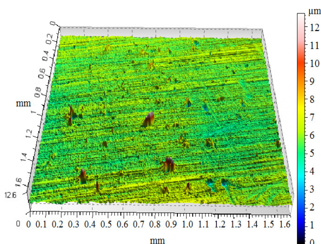
Fig. 8. 3D optical surfaces of the sample before machining. S_a = 0.3501 \mu\text{m}
