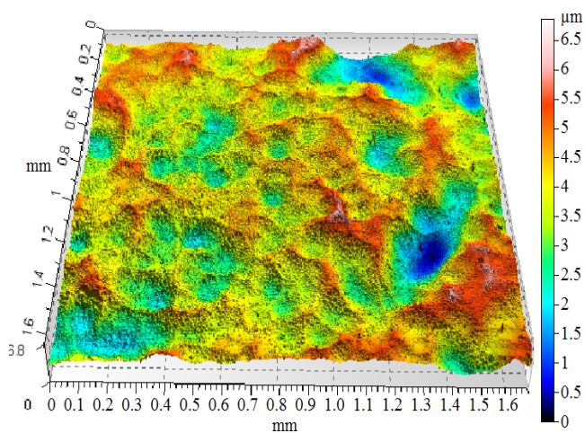
Fig. 10. 3D optical surfaces of the sample after vibro-polishing on 60 min; S_a = 0.7074 \mu\text{m}
