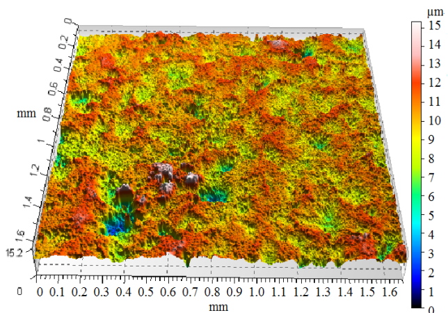
Fig. 9. 3D optical surfaces of the sample after vibro-abrasive deburring on 60 min; S_a = 1.0163 \mu\text{m}
