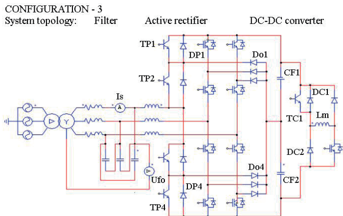
Fig. 7. Mixed configuration with two-level DC-DC converter and three-level 3-phase active rectifier
