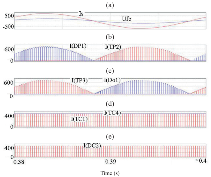
Three-level rectifier a) I_s – interface input phase current, THDI_s = 1.35\% , U_{fo} – interface input phase voltage, THDU_{fo} = 1.15\% , b) I(Tp2) – rectifier transistor current, I(Dp1) – rectifier diode current, c) I(Tp3) – rectifier transistor current, I(Do1) – rectifier zero diode current, Two-level DC-DC converter d) I(TC1) – converter transistor current, I(TC4) – converter transistor current, e) I(DC2) – converter diode current.
