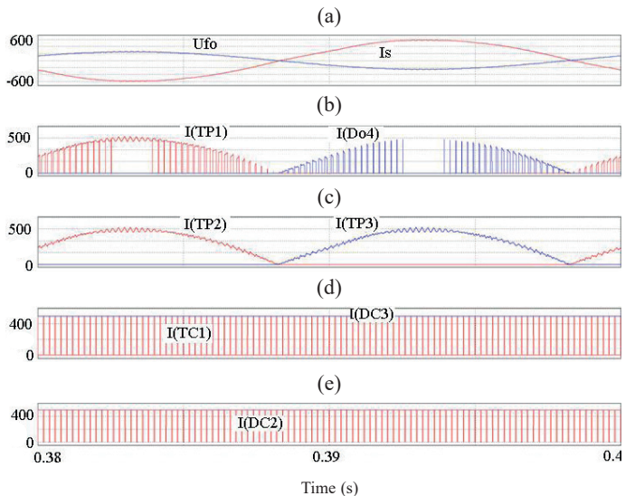
Three-level rectifier a) I_s – interface input phase current, THDI_s = 1.77\% , U_{fo} – interface input phase voltage, THDU_{fo} = 1.41\% , b) I(Tp1) – rectifier transistor current, I(Do4) – rectifier zero diode current, c) I(Tp2) – rectifier transistor current, I(Tp3) – rectifier transistor current, Two-level DC-DC converter d) I(TC1) – converter transistor current, I(DC3) – converter diode current, e) I(DC2) – converter diode current.
