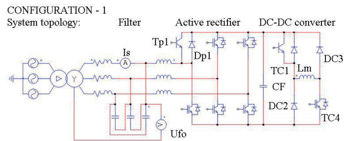
Fig. 1. Circuit configuration with two-level DC-DC converter and two-level 3-phase active rectifier
