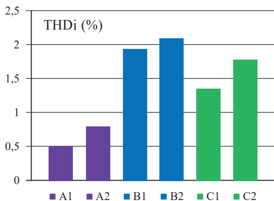
Fig. 10. Total harmonic distortion – current THD_i
