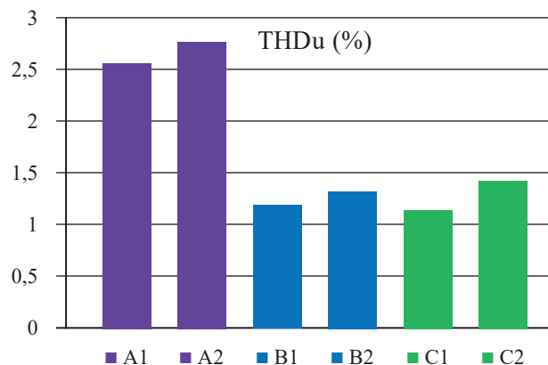
Fig. 11. Total harmonic distortion – voltage THD_u
