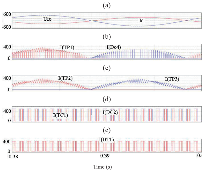
Three-level rectifier a) I_s – interface input phase current, THDI_s = 2.09\% , U_{fo} – interface input phase voltage, THDU_{fo} = 1.29\% , b) I(Tp1) – rectifier transistor current, I(Do4) – rectifier zero diode current, c) I(Tp2) – rectifier transistor current, I(Tp3) – rectifier transistor current, Three-level DC-DC converter d) I(TC1) – converter transistor current, I(DC2) – converter diode current, e) I(DT1) – converter zero diode current.
