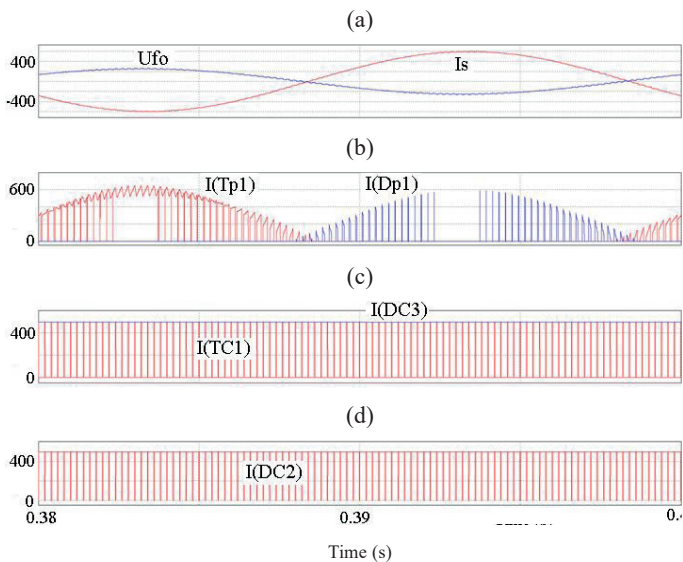
Fig. 5. Energy flow from the power network to the storage reactor in three-level topology
