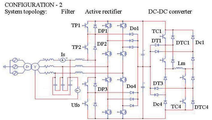
Fig. 4. System topology with three-level DC-DC converter and three-level 3-phase active rectifier
