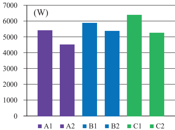
Fig. 14. Total power losses in the semiconductor components for all interface topologies
