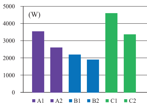
Fig. 12. Power losses in the active rectifier
