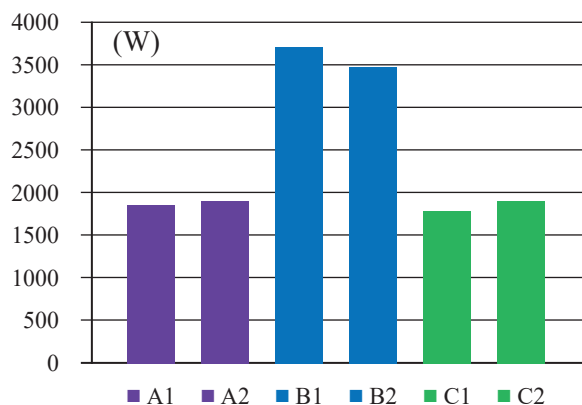
Fig. 13. Power losses in the DC-DC converter
