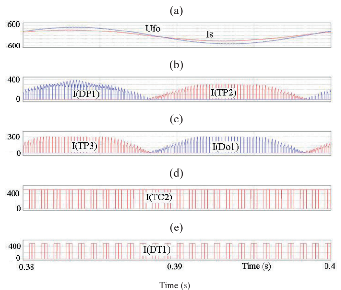
Fig. 2. Energy flow process from the power network to the storage reactor in two-level topology
