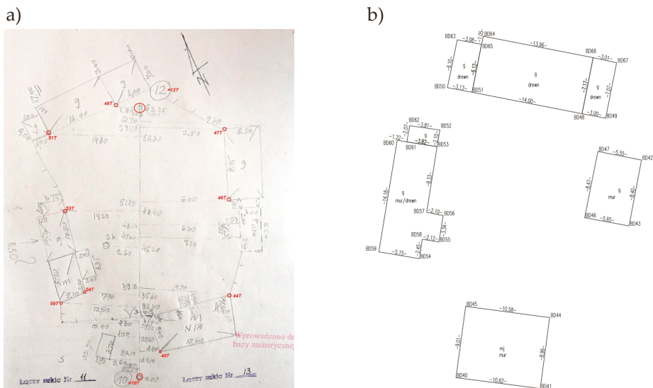
Fig. 8. Field sketch of building – base map updating measurement: Warsaw's West District Geodetic and Cartographic Resources (a) and author's GNSS control measurement field sketch (b)
