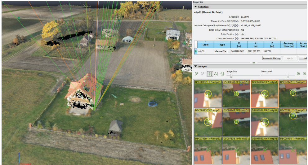
Fig. 10. Multiple space intersections on a 3D model (Pix4D software)
