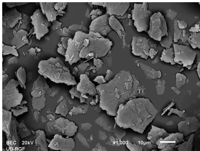
Fig. 7. Microphotograph of refractory fillers based on talc
