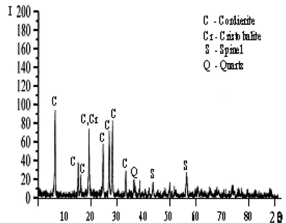
Fig. 2. Diffractograms of the filler based on cordierite
