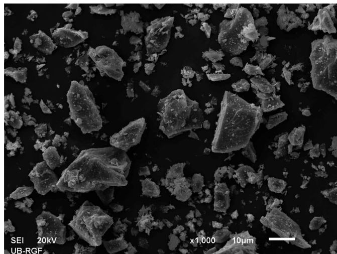
Fig. 8. Microphotograph of refractory fillers based on cordierite
