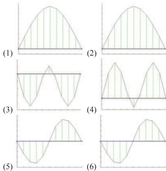
Fig. 7. Mode shapes for the base model, \alpha = 3,0 ; \beta = 0,000005 .
