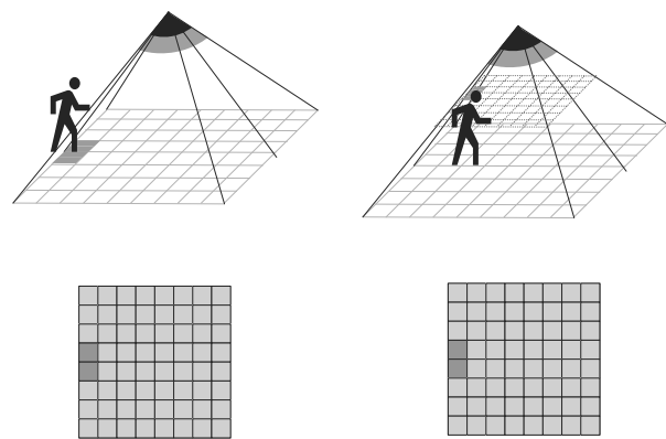
Fig. 2. Gait speed errors caused by cone-shape signals.
