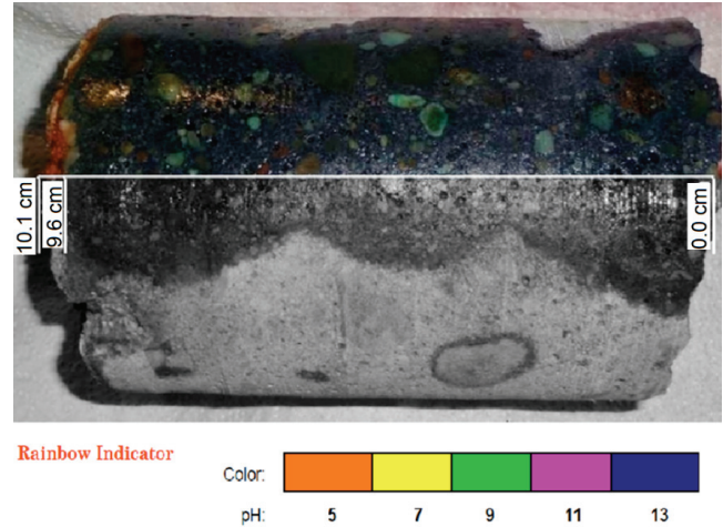
Fig. 3. Carbonation zone identification using chemical indicator
