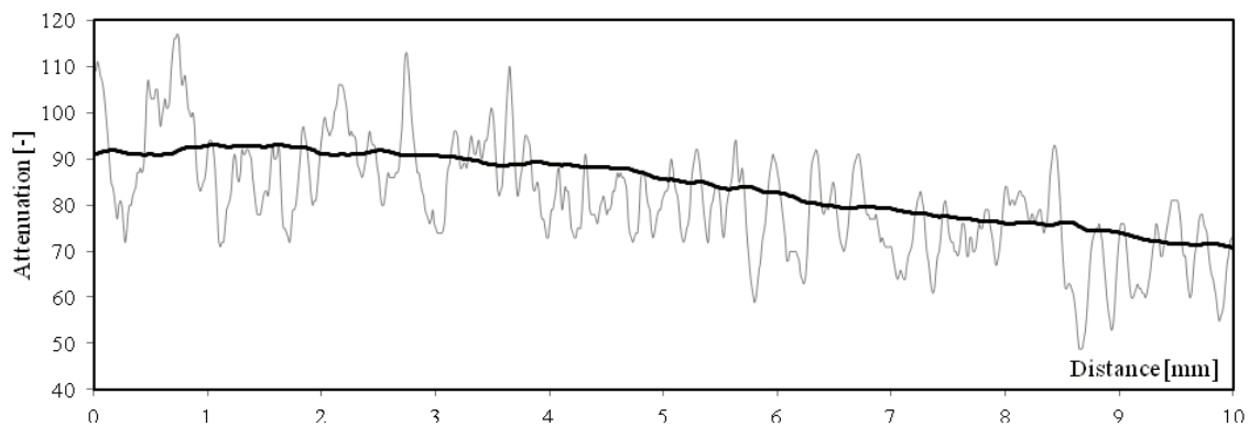
Fig. 10. Attenuation curve on the height of the sample after second scanning
