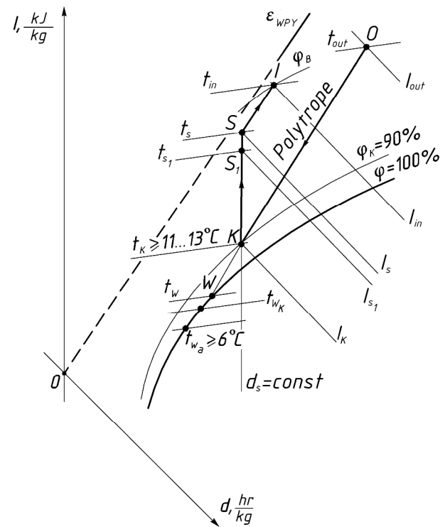
Fig. 2. The image of the process of changing the moist air state in the straight flow air conditioning system in a warm period of year on the I-d diagram: OK – the process of polytropic air treatment (cooling and drying) G_{a.w} = G_S in the air washer; KS_1 – the air G_S heating process in the air heater of second heat; S_1S – the air G_S heating by 1^\circ\text{C} in the fan and the supply air duct; SI – the process of excess heat and moisture assimilation in the cleanroom by the supplied air G_S via the air conditioner
