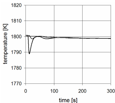
Fig. 2b. Change in temperature of the liquid steel in selected measurement points P1, P2 and P3 for addition size of 45 kg and argon flow rate of 200 l/min
