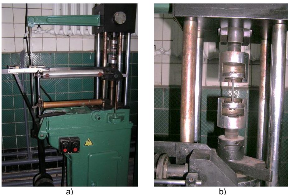
Fig. 1. Test of specimens in testing machine IM 4P: a) general view, b) specimen it testing
