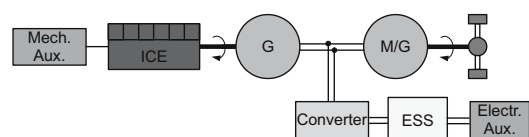
Fig. 1. Architecture of a hybrid diesel-electric railway vehicle.
