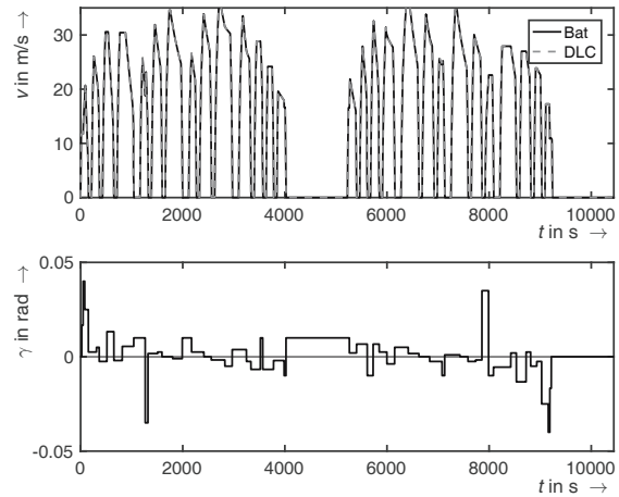
Fig. 7. Reference trajectory.
