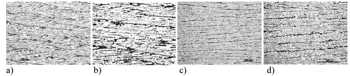
Fig. 4. Microstructure of directionally solidified Fe-Fe 3 C eutectic alloy on the longitudinal section of each samples, G = 33,5 \text{ K/mm} , a,b) v = 83,3 \mu\text{m/s} , c,d) v = 166,7 \mu\text{m/s}
