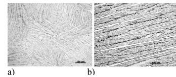
Fig. 5. Microstructure of a) eutectic, b) hypereutectic structure areas - samples after solidifying was frozen (immediately taken off the cooler), v = 83,3 \mu\text{m/s} , G = 33,5 \text{ K/mm}
