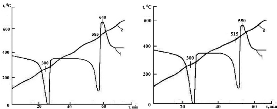
Figure 1. Thermograms of the decomposition of neat PP (left) and PP containing 3 wt.% copper(II) oxide (right). The DTA and temperature curves are labelled as curves 1 and 2 respectively
