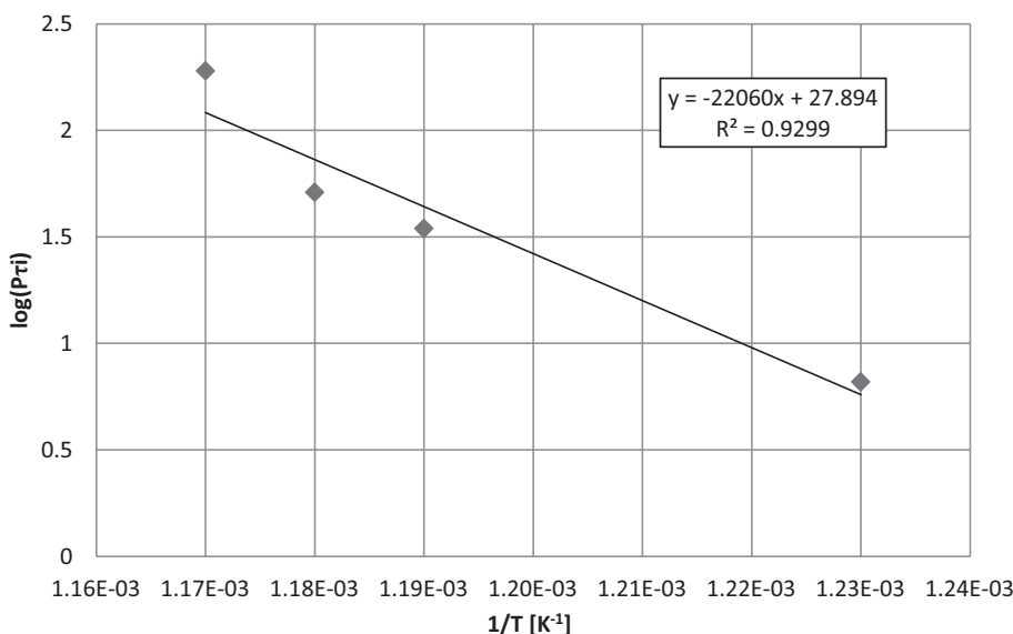
Figure 2. The semi-logarithmic dependence of the change of PP decomposition rate on the inverse temperature plot
