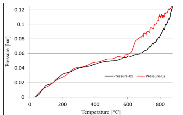
Fig. 8. Dependency graph pressure - temperature - sample number 4
