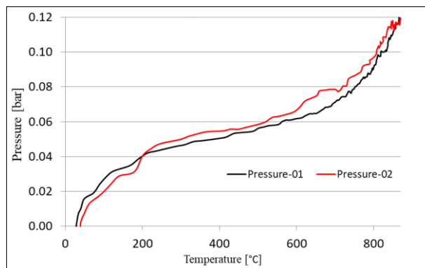
Fig. 10. Dependency graph pressure - temperature - sample number 6
