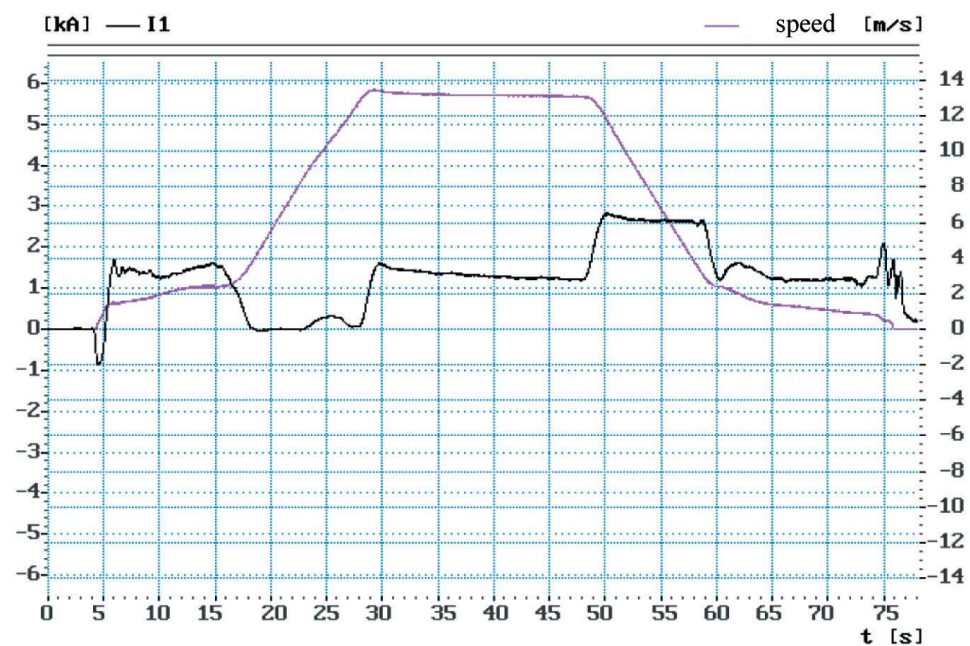
Fig. 6. Randomly selected speed registrations – correct operation of the hoisting machine after the introduced changes
