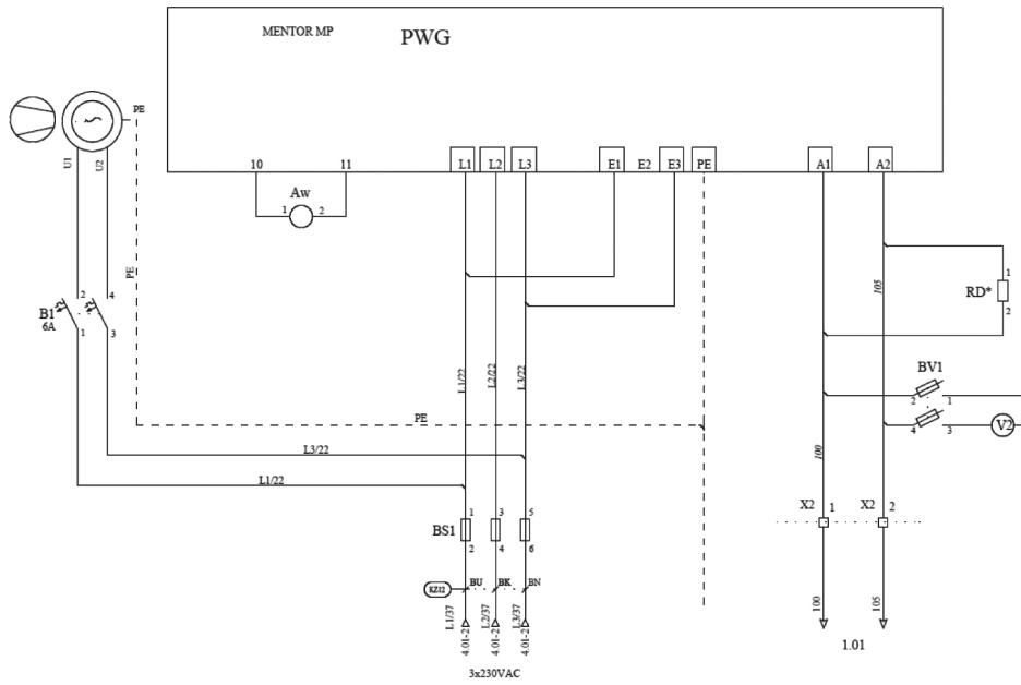
Fig. 4. Excitation of the control generator [4]
