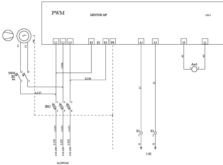
Fig. 5. Excitation of the driving motor of the hoisting machine [4]
