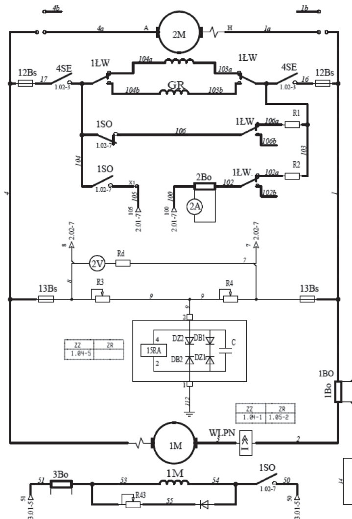
Fig. 3. Schematic diagram of the hoisting machine drive after introduced changes [4]
