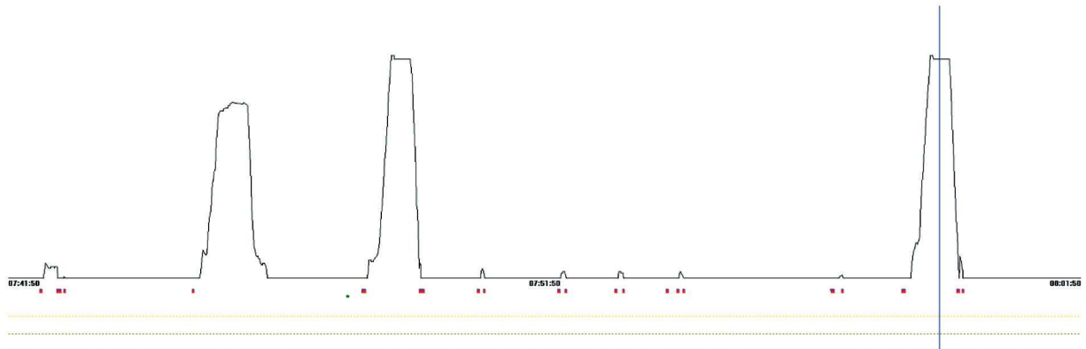
Fig. 2. Randomly selected recording of the travel speed – incorrect operation of the hoisting machine
