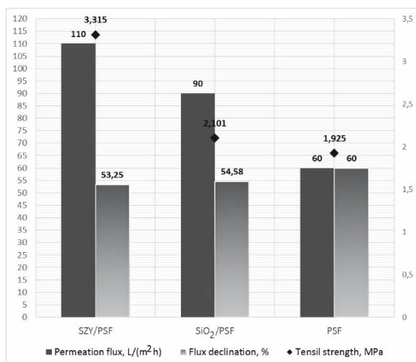
Fig. 2. Utility parameters of polysulfon membranes (PSF), on the basis of (Zhang et al. 2011)
