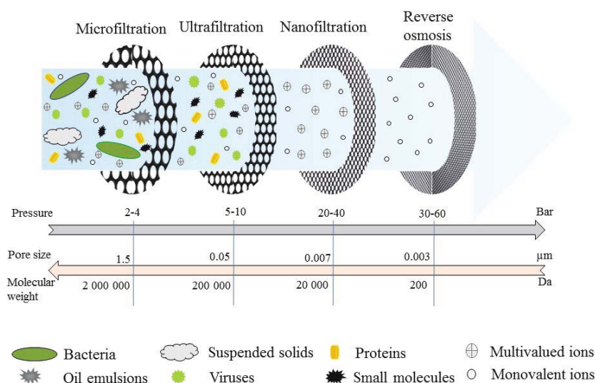
Fig. 1. Comparison of pressure filtration methods (own analysis)
