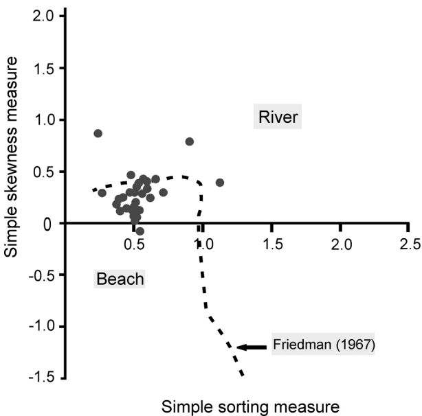
Fig. 12. Bivariate plot depicting environment of deposition simple sorting measure (SOS) vs simple skewness measure (SKS)
