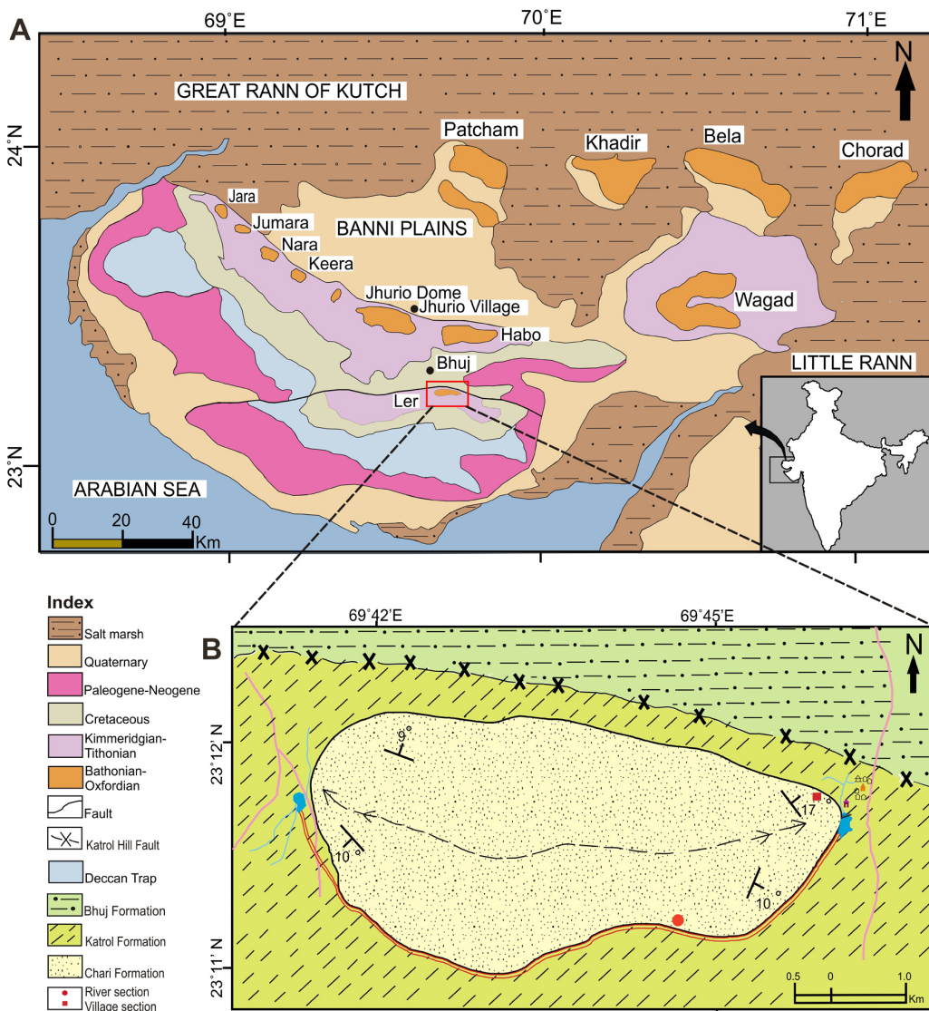
Fig. 1. A – Geological map of the Kachchh Basin (from Fürsich et al., 2001); B – Geographical extension of the Ler Dome in western India (after Ghaznavi et al., 2015)
