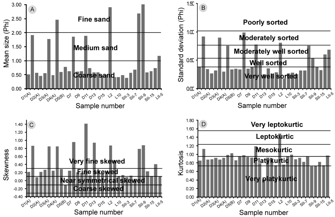
Fig. 6. Histograms of all samples plotted with respect to statistical parameters calculated by the graphical method: A – Mean grain size; B – Standard deviation; C – Skewness; D – Kurtosis
