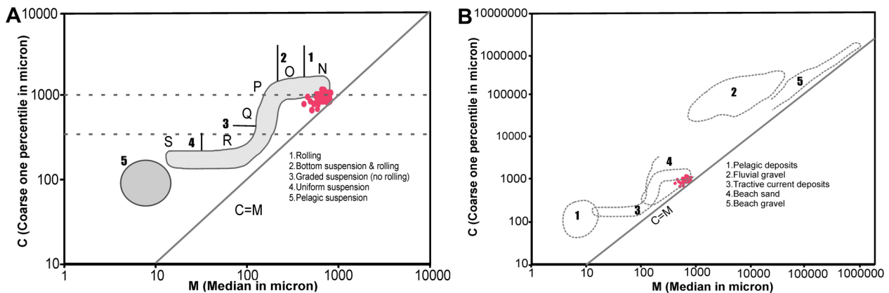
Fig. 14. CM plot to determine depositional mechanisms (A) and sedimentary subenvironments (B) of the Dhosa sandstones (after Passega, 1957, 1964)
