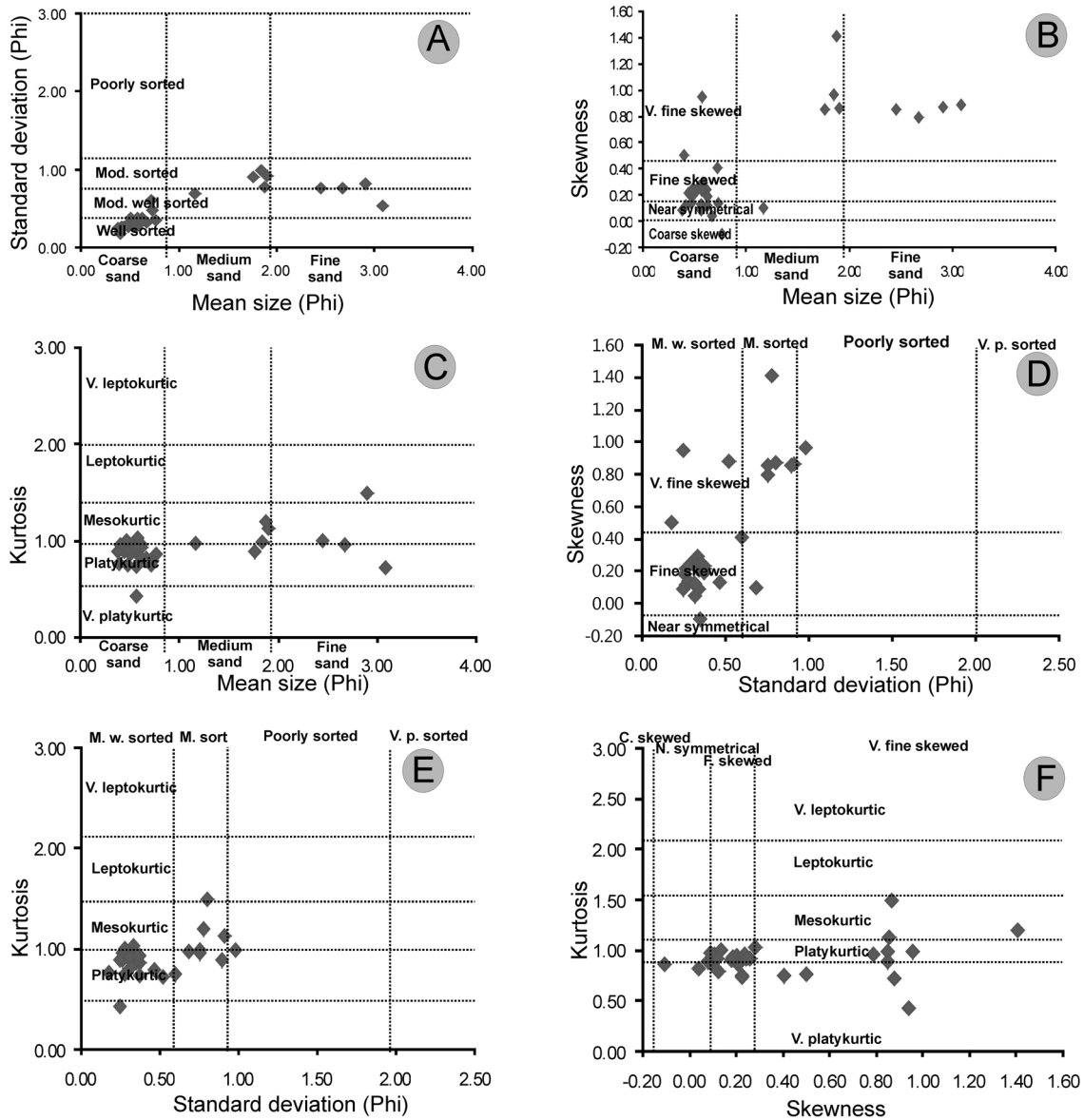
Fig. 8. Sector plot showing the bivariate relationship between: A – Grain size and sorting; B – Grain size and skewness; C – Grain size and kurtosis; D – Sorting and skewness; E – Sorting and kurtosis; F – Skewness and kurtosis
