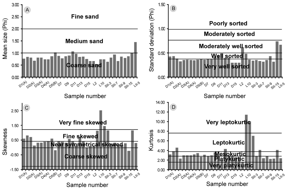
Fig. 7. Histograms of all samples plotted with respect to statistical parameters calculated by the moment method: A – Mean grain size; B – Standard deviation; C – Skewness; D – Kurtosis
