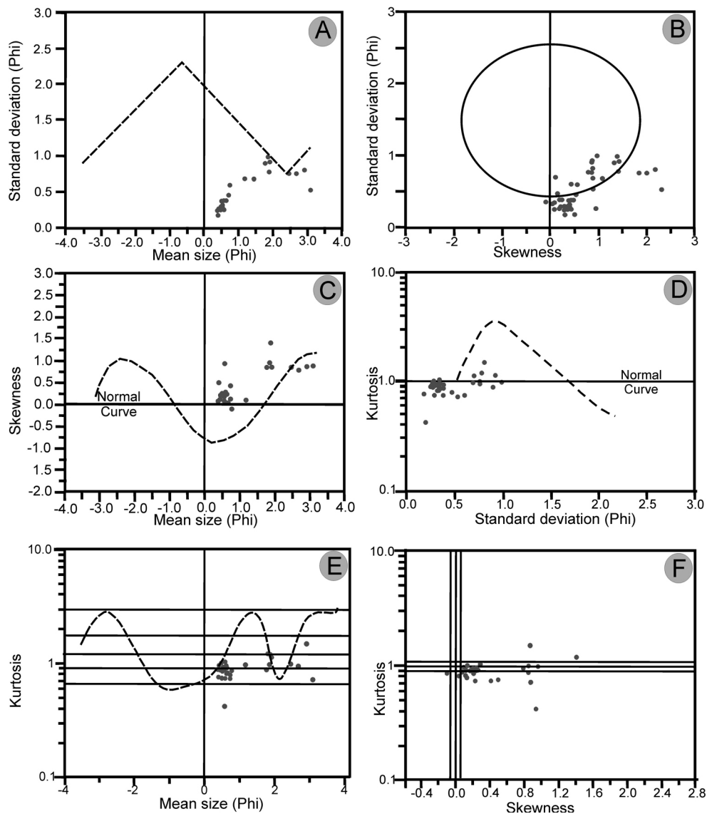
Fig. 9. Bivariate plots showing the placement of the present samples in the model plot as proposed by Folk & Ward (1957). A – Mean grain size vs standard deviation; B – Skewness vs standard deviation; C – Mean grain size vs skewness; D – Standard deviation vs kurtosis; E – Mean grain size vs kurtosis; F – Skewness vs kurtosis
