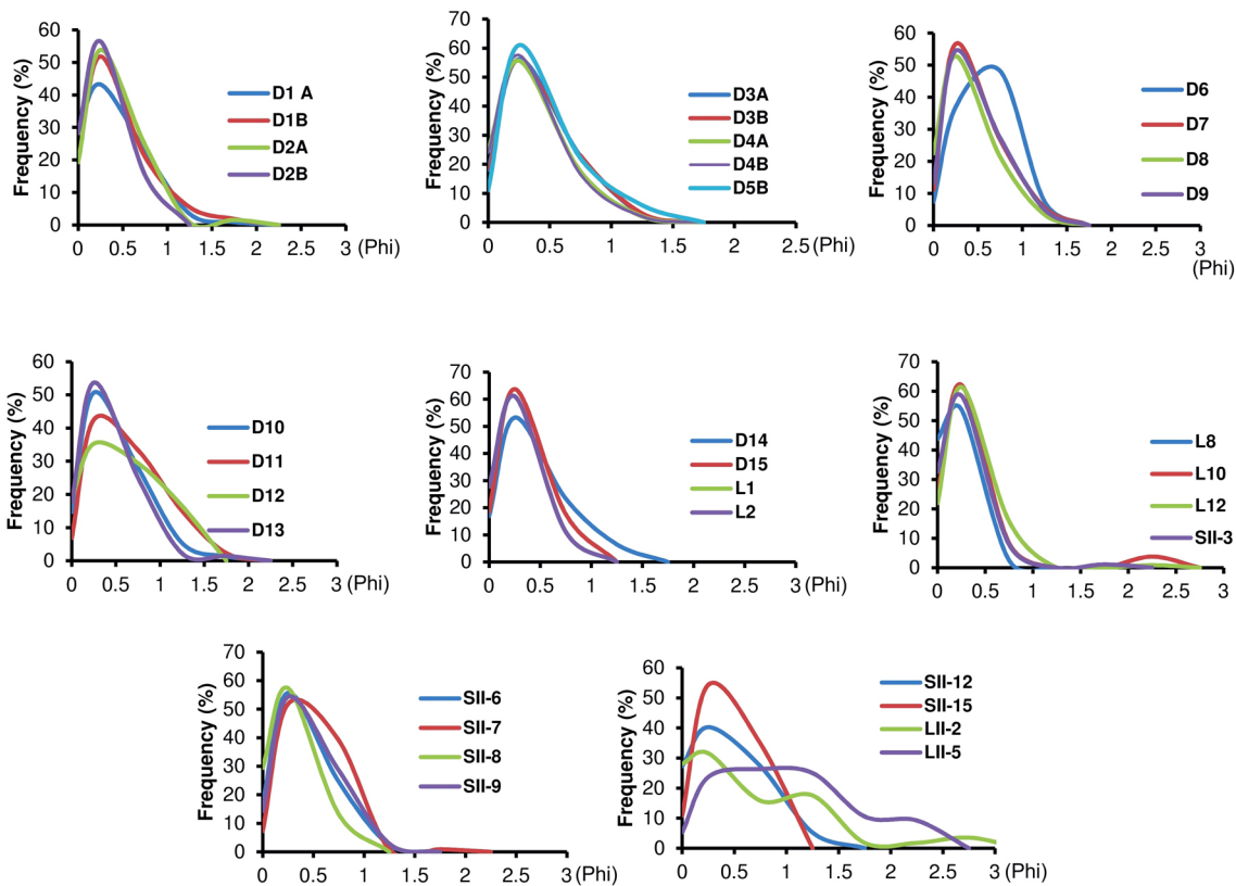
Fig. 4. Grain size distribution curves for the Dhosha sandstones
