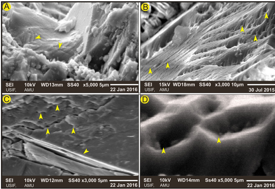
Fig. 3. Microstructures in quartz grains from Dhosha Sandstone as observed in scanning electron micrographs: A - Grooves; B - Straight steps and V-shaped pits; C - Curved and straight steps in association with silica precipitation; D - Solution pits
