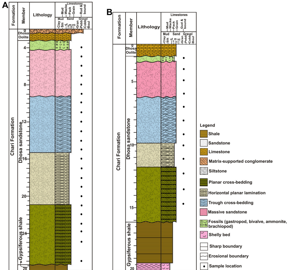
Fig. 2. Lithostratigraphical columns showing the various lithofacies of the Ler Dome, Kachchh, exposed at: A - river section (after Ghaznavi et al., 2018b); B - village section
