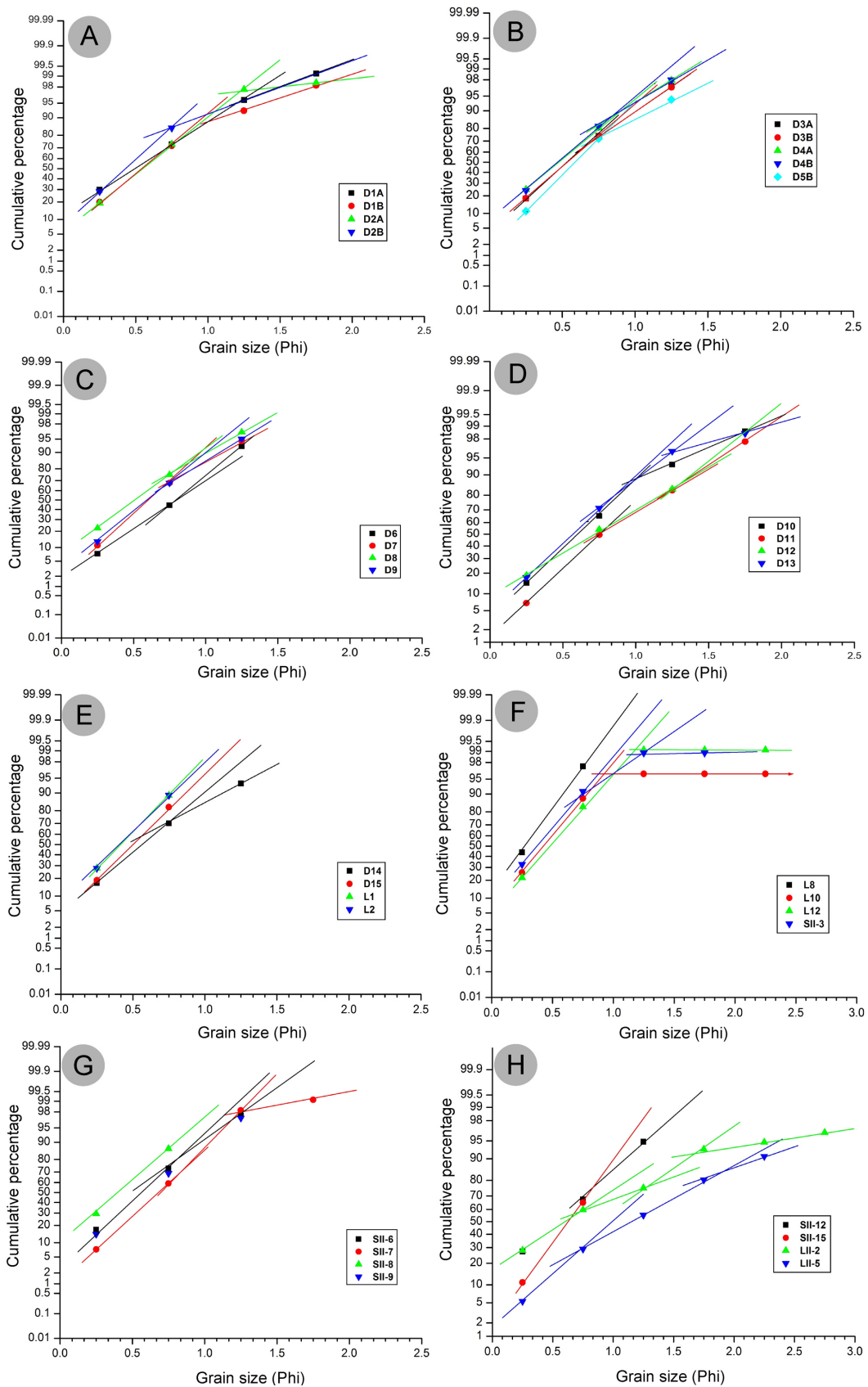
Fig. 15. Log probability curves showing the trend of traction, saltation and suspension population of all samples (after Visher, 1969)
