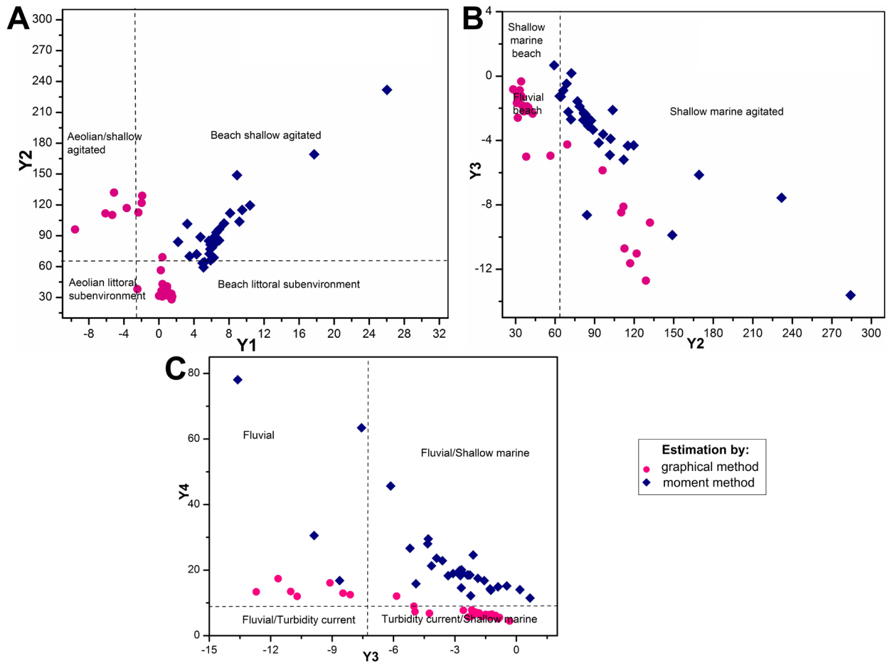
Fig. 13. Linear discriminate function plot for Dhosa sandstones. A – Y_1 vs Y_2 discriminates between beach and aeolian environment; B – Y_2 vs Y_3 discriminates between beach and shallow-marine subenvironment; C – Y_3 vs Y_4 discriminates between marine turbidity and fluvial environment
