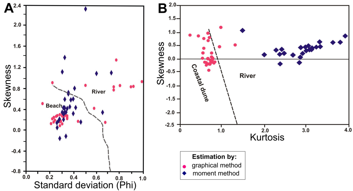
Fig. 11. A - Bivariate plot of skewness vs inclusive graphic standard deviation (after Friedman, 1967); B - Bivariate plot of skewness vs kurtosis (after Folk & Ward, 1957)
