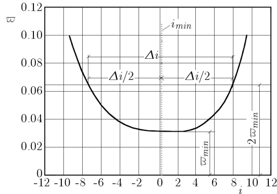
Fig. 2. Illustration of the reference condition
