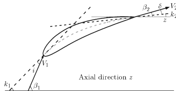
Fig. 3. The correlations between cascade and aerodynamics parameters
