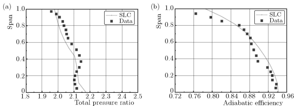
Fig. 4. Total pressure ratio (a) and adiabatic efficiency (b) for 0.98 mass flow rate
