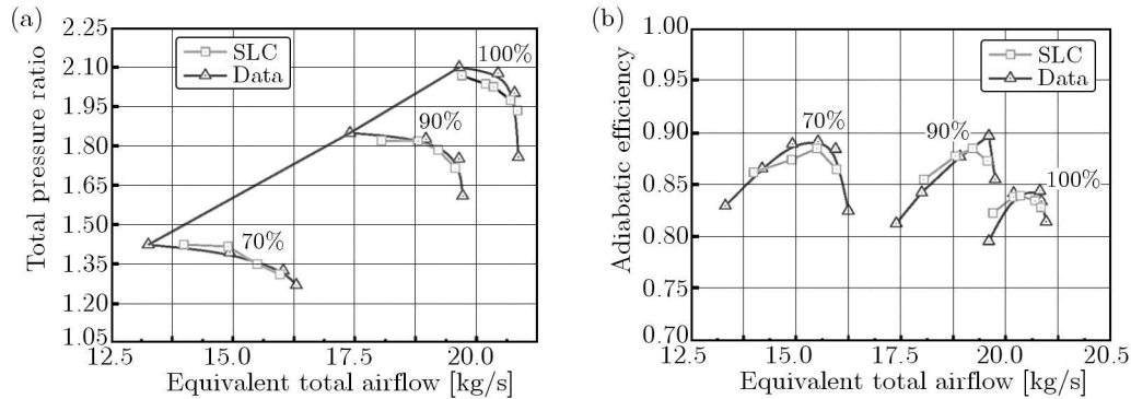
Fig. 7. Performance curve of pressure ratio (a) and of adiabatic efficiency (b) for the compressor
