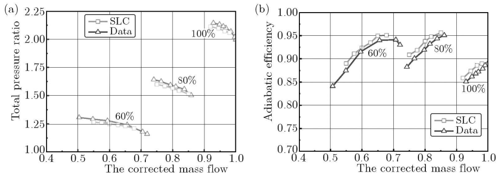
Fig. 6. Performance curve of pressure ratio for the rotor (a) and of adiabatic efficiency for the rotor (b)
