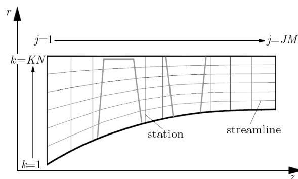
Fig. 1. The computational grids in the meridian plane
