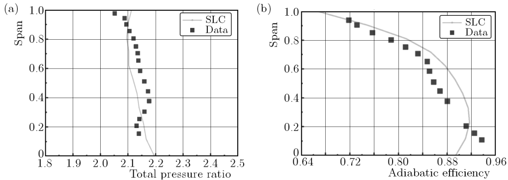
Fig. 5. Total pressure ratio (a) and adiabatic efficiency (b) for 0.92 mass flow rate
