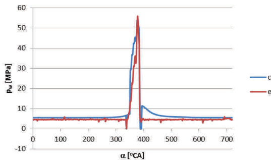
Fig. 10. The pressure course of in the injection pump measured in experimental studies (e) and calculated (c) for the 100% of the engine load
