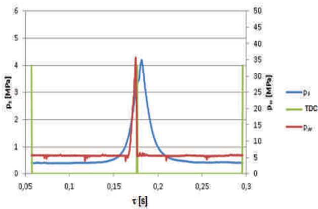
Fig. 3. Course of the pressure in a combustion chamber and the injection pump of the cylinder for one cycle at engine load of the 0%: p_s – pressure course in the combustion chamber, TDC – top dead centre, p_w – pressure in the injection pump
