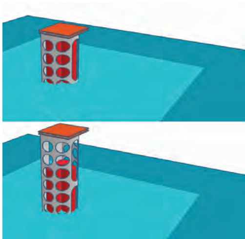
Fig. 11. The wave energy absorber submerged in water in a test tank – top dead centre position on the top and bottom dead centre position on the bottom.
