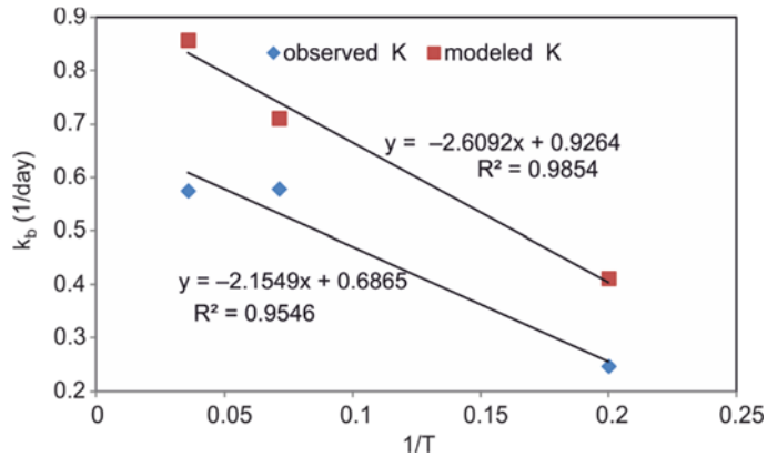
Fig. 4. Reaction rate constant of \text{Cl}_2 decay ( k_b ) as a function of temperature
