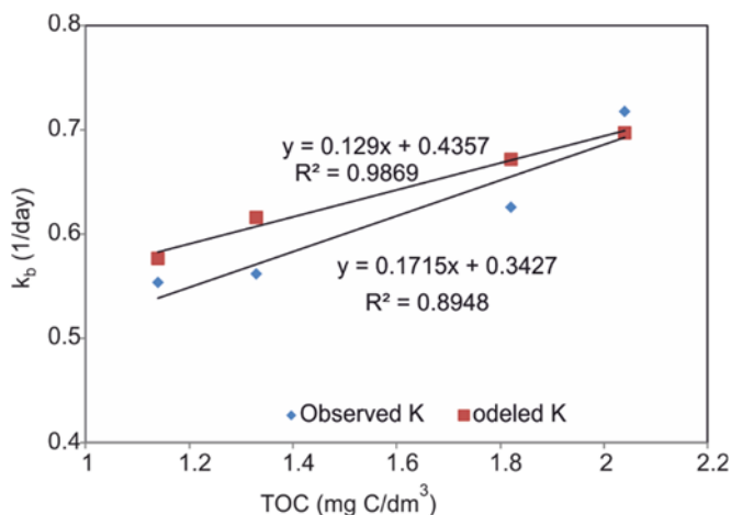
Fig. 6. Reaction rate constant of \text{Cl}_2 decay ( k_b ) as a function of TOC
