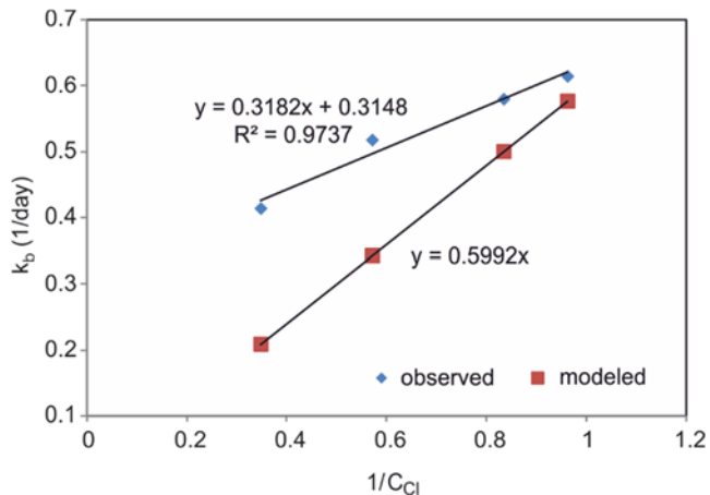
Fig. 5. Reaction rate constant of \text{Cl}_2 decay ( k_b ) as a function of C_{\text{Cl}}
