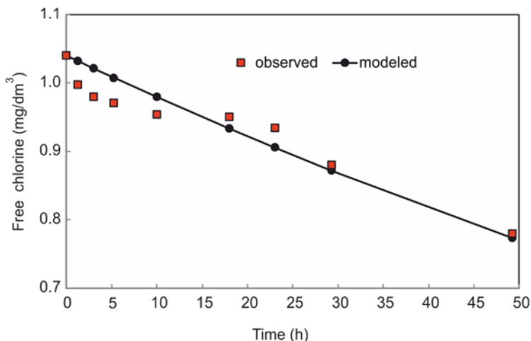
Fig. 1. Regression of \text{Cl}_2 decay kinetics for drinking water at 5^\circ\text{C} , pH 7.8, TOC 1.14 \text{ mg C/dm}^3 , and [\text{Br}^-] 42 \mu\text{g/m}^3
