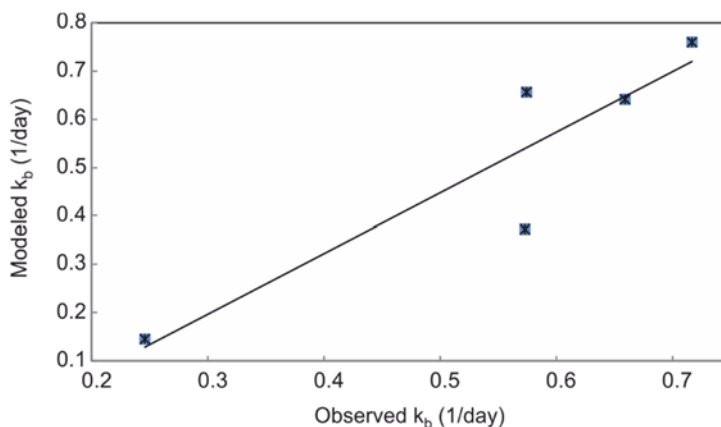
Fig. 2. Modeled and observed k_b values based on Eq. (3) k_b modeled using Eq. (3) with the following constants: e = 5501.8^\circ\text{C} , a = 4.977 \times 10^6 , b = 0.6478173 , R^2 = 0.8308
