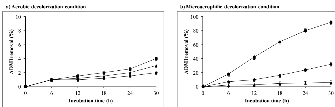
Fig. 2. Decolorization of textile effluent by individual A. ochraceus NCIM 1146 (—▲—), P. rettgeri strain HSL1 (—●—) and their fungal-bacterial consortium (—■—) under a) aerobic, and b) microaerophilic conditions (Data points indicate the mean of three independent replicates, standard error of mean is indicated by error bars)
