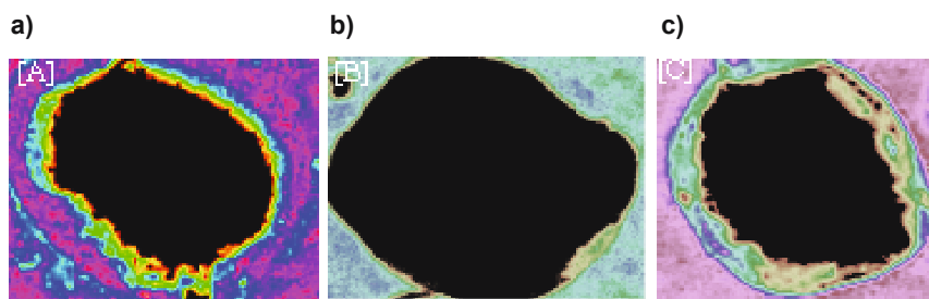
Fig. 5. Analysis of comets observed a) control as treated with distilled water, b) treated with textile effluent, and c) treated with degradation metabolites of textile effluent after treatment with fungal-bacterial consortium under microaerophilic conditions
