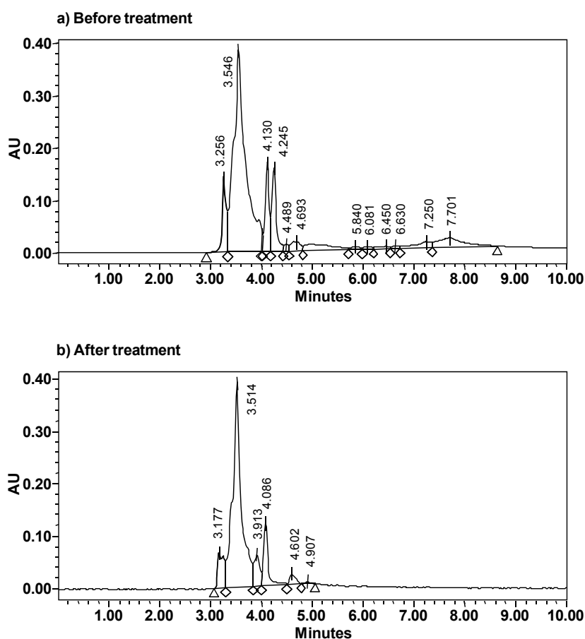
Fig. 4. HPLC elution profile of a) untreated textile effluent, and b) its decolorization metabolites obtained after treatment with fungal-bacterial consortium under microaerophilic conditions
