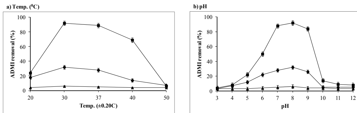
Fig. 3. Effect of a) incubation temperature and b) pre-grown culture medium pH on decolorization of textile effluent by individual A. ochraceus NCIM 1146 (—▲—), P. rettgeri strain HSL1 (—●—) and fungal-bacterial consortium (—■—) under microaerophilic conditions (Data points indicate the mean of three independent replicates, standard error of mean is indicated by error bars)
