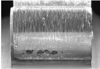
Fig. 4. Pitting in the HCR gearing Rys. 4. Pitting w uzębieniu HCR
