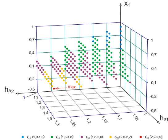
Fig. 7. Optimal values h_{a1}^* , h_{a2}^* , X_1 for maximum contact load capacity depending on \varepsilon_\alpha
