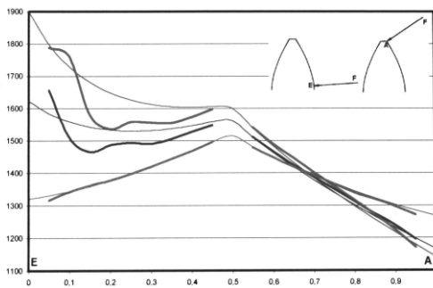
Fig. 6. Contact stress of HCR gears along the contact path for various geometry characteristics of gearing
