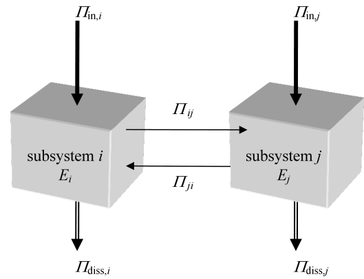
Fig. 3. Two subsystem SEA model.
