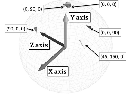
Fig. 1. Sphere of rotation to visualize rotational data sets (Jabłoński, 2008a).
