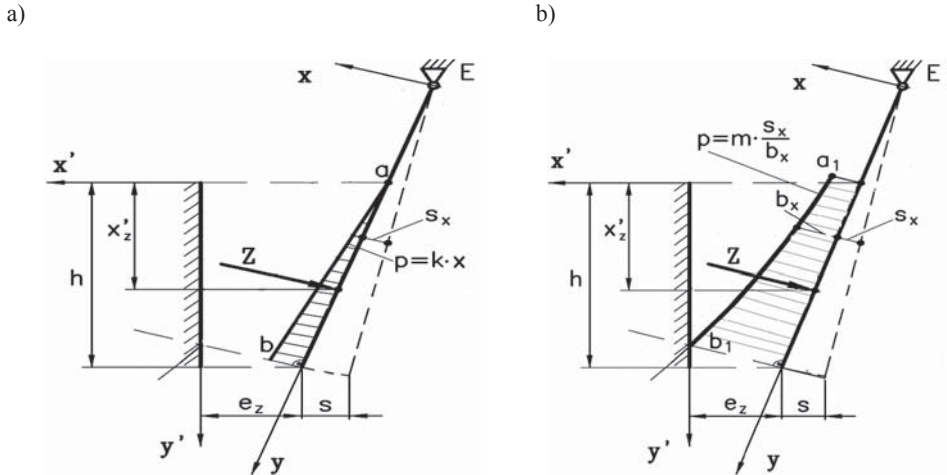
Fig. 3. Load diagram recommended for calculations a) linear p = kx , b) non-linear p = mS_x/b_x^3 , m - constant of proportionality [3, 8–10]
