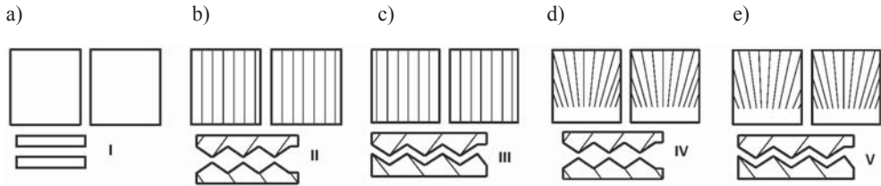
Fig. 2. Crushing plates used in laboratory tests
