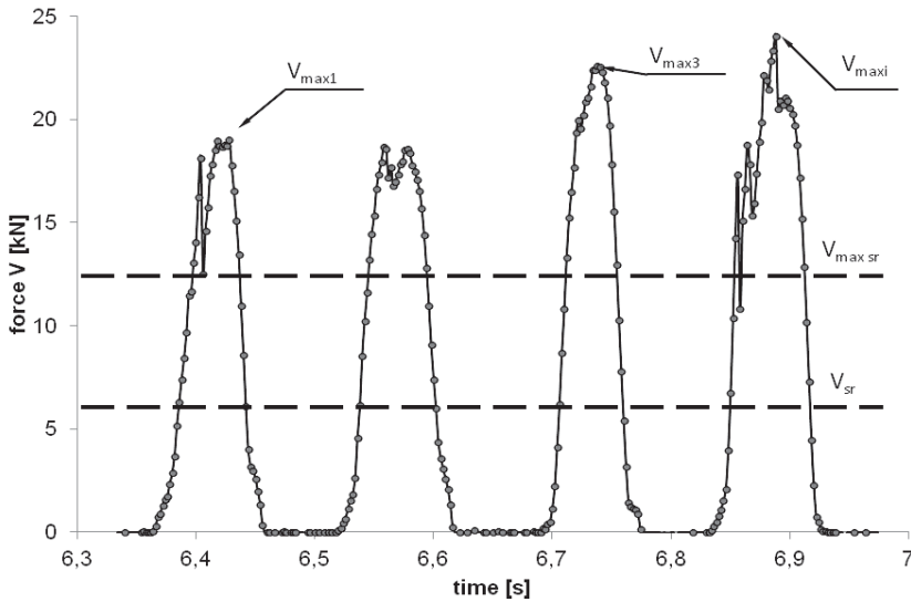
Fig. 6. The determination of normal forces V average values V_{sr} and V_{\max sr} mean values from one test are shown
