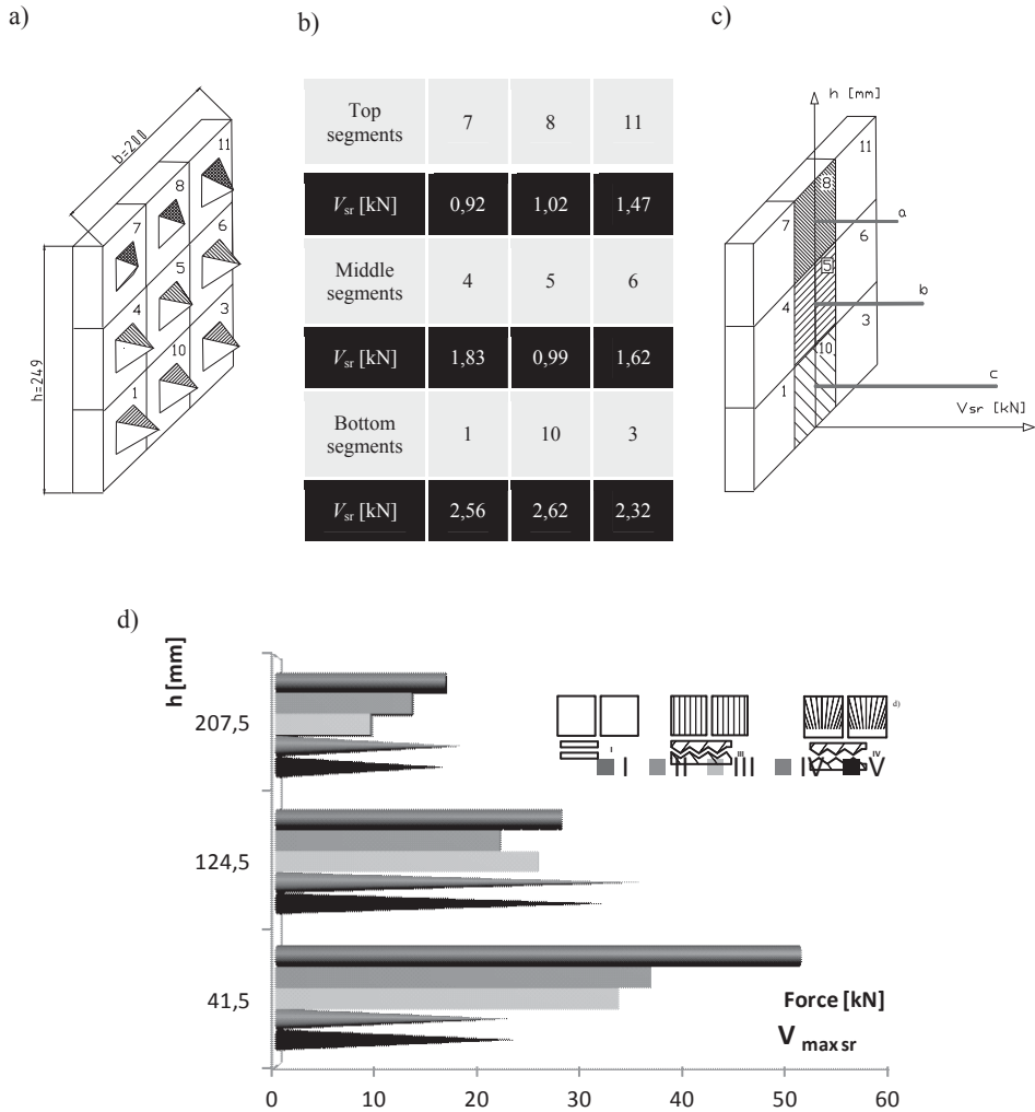
Fig. 7. Crushing process on flat plates: a, b) values of V_{sr} forces acting on each segment in the series, c) fixed plate with coordinates, d) mean maximum values of normal V_{max\ sr}
