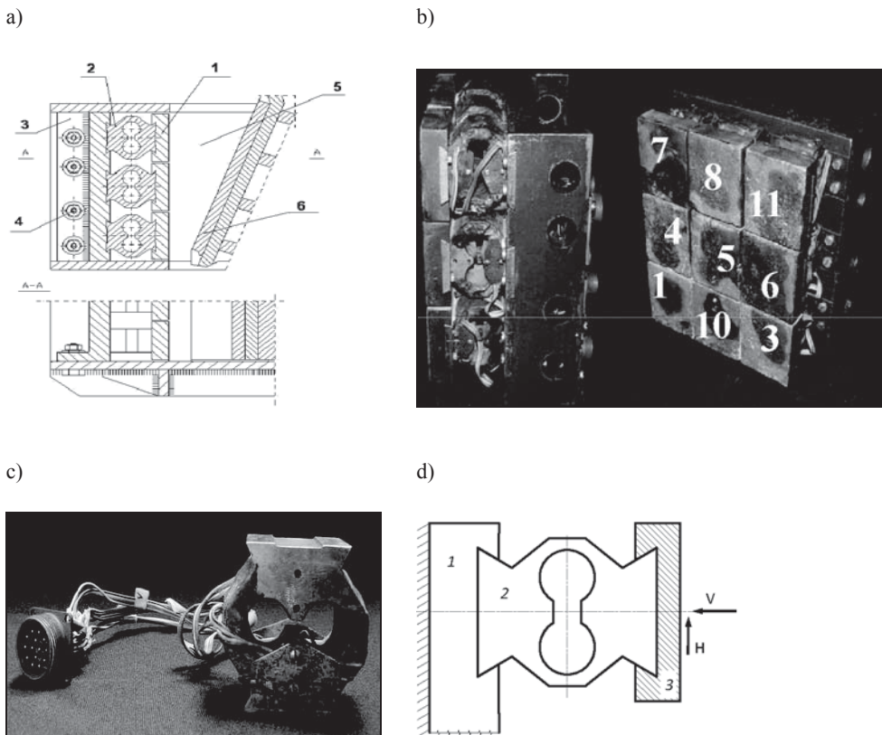
Fig. 1. Force measurement in the crusher working space:
