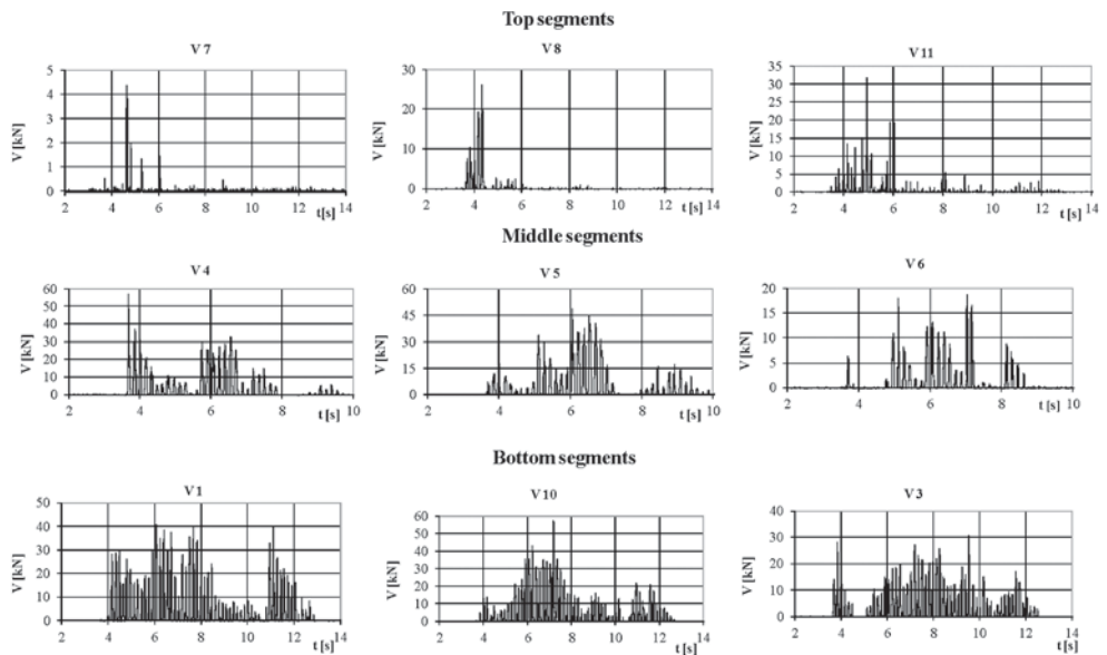
Fig. 4. Sample graphs of normal force changes V ( V1 , V2 , V3 , etc.), acting on each segment of fixed crushing plate (first series of tests)
