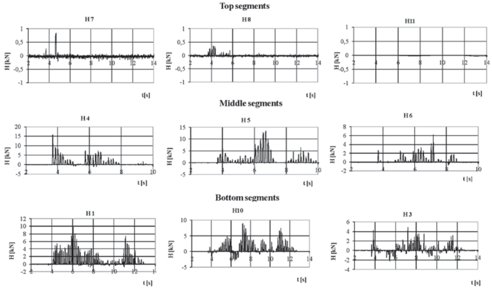
Fig. 5. Sample graphs of tangential force changes H ( H1 , H2 , H3 , etc.), acting on each segment of fixed crushing plate (first series of tests)
