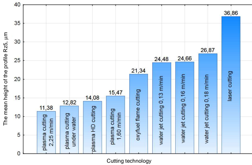
Fig. 9. Results of the mean height of the profile Rz5 measurements
